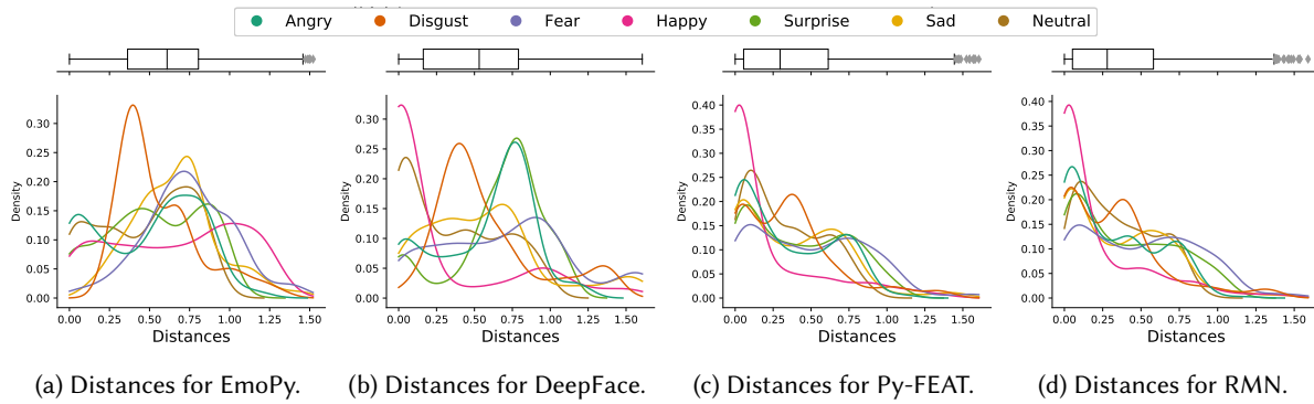
Fig. 17. Illustration of the distance distribution for each emotion on AffectNet images.
