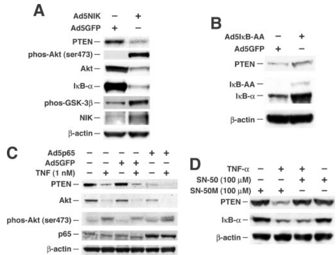
FIG. 3. NIK and activation of p65 NF- \kappa B decrease PTEN expression. A , adenoviruses (Ad5NIK) carrying the NIK gene were infected into HT29 cells at a multiplicity of infection of 20. Ad5NIK-infected cells were compared with cells infected with control adenovirus (Ad5GFP) carrying green fluorescence protein. After a 48-h incubation, attached cells were collected and proteins extracted for Western blot analysis. PTEN expression was found to be lower for Ad5NIK-infected cells. In addition, a decrease in total Akt and I \kappa B- \alpha expression but an increase in phospho-Akt (Ser-473) and phospho-GSK-3 \beta levels were observed for Ad5NIK-infected cells. NIK overexpression was confirmed for Ad5NIK-infected cells. B , HT29 cells were infected with Ad5I \kappa B-AA, which contains the superrepressor I \kappa B- \alpha gene, at a multiplicity of infection of 20. Western blot analysis shows expression of I \kappa B-AA, which has a higher molecular weight than endogenous I \kappa B- \alpha because of hemagglutinin protein attachment. Ad5I \kappa B-AA infection increased PTEN and I \kappa B- \alpha expression consistent with results obtained as in A . C , adenovirus Ad5p65 carrying the p65 subunit of NF- \kappa B was infected into HT29 cells at a multiplicity of infection of 20. Ad5GFP was used as control infection. After 48 h postinfection, attached cells were collected for Western blot analysis. Ad5p65 infection decreased PTEN and Akt expression but increased phospho-Akt expression similar to the result with Ad5NIK infection. Anti-p65 blotting shows p65 overexpression for Ad5p65-infected cells. D , HT29 cells were pretreated with cell membrane-permeable SN50 peptide that binds to unbound NF- \kappa B 30 min prior to TNF- \alpha treatment. SN50M, a mutant variant of SN50 which does not bind to NF- \kappa B, was used as control peptide. After a 24-h incubation with TNF- \alpha and SN50, attached cells were collected and proteins extracted for Western blot analysis. SN50 completely blocked TNF- \alpha -induced reduction in PTEN expression, whereas SN50M had no effect. The I \kappa B- \alpha level was decreased for TNF- \alpha - and SN50-treated cells as expected because SN50 does not prevent TNF- \alpha -mediated I \kappa B- \alpha degradation. Equal \beta -actin shows even loading of proteins.
