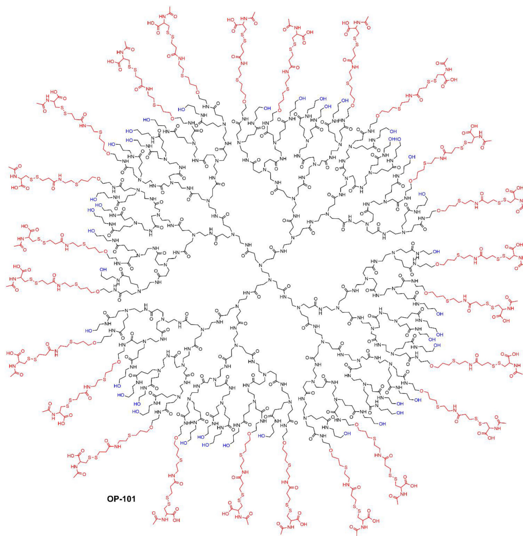
Figure 3. Hydroxyl generation 4 PAMAM dendrimers stochastically functionalized; one of the possible full structure of OP-101.
