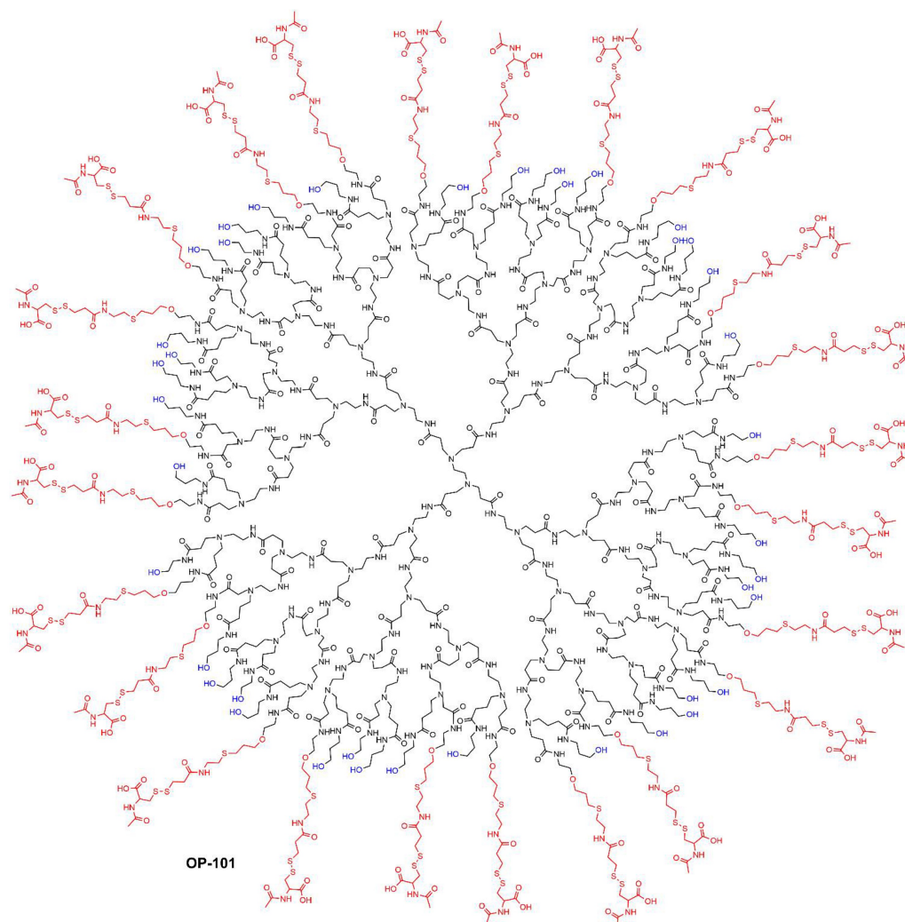
Figure 3. Hydroxyl generation 4 PAMAM dendrimers stochastically functionalized; one of the possible full structure of OP-101.
