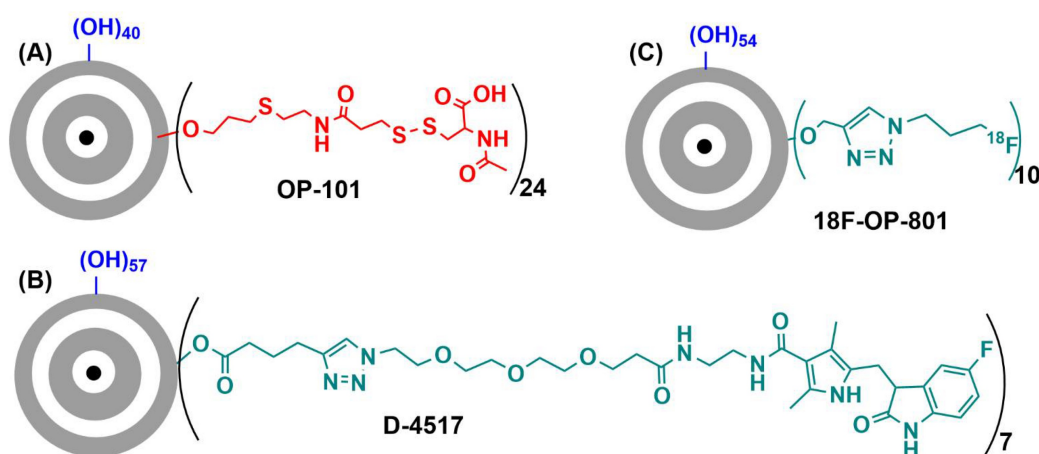
Figure 4. (A) Simplified structure of OP-101. (B) Simplified structure of D-4517. (C) Simplified structure of 18F-OP-801.
