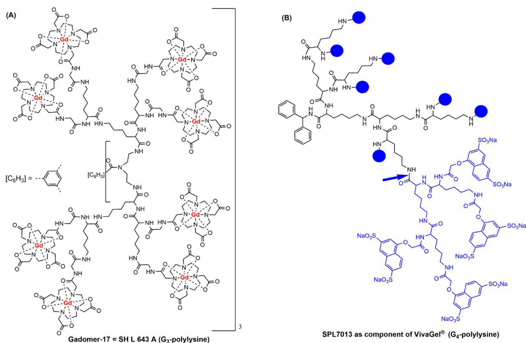
Figure 1. Chemical structure of two poly-L-Lysine dendrimers. (A) Gadomer-17 used as MRI agent. (B) SPL7013, also named Astodrimer sodium, the active ingredient in the mucoadhesive gel
