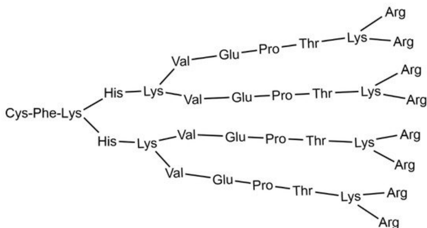
Figure 5. Structure of the cationic peptide dendrimer KK-46, usable as carrier of siCoV.
