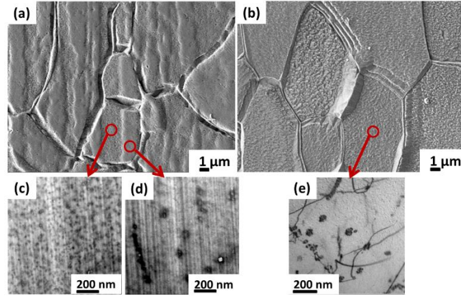
Fig. 11. SEM images of a specimen of IF steel double side coated with 500 nm thick FeC film after induction heating at 780 °C – 2 minutes (a) and at 780 °C – 4 minutes (b). BF-STEM images obtained with TEM in a zone inside the bands (c) and surrounding the bands (d) for the specimen kept at 780 °C for 2 minutes. (e) BF-STEM image inside a grain for specimen kept at 780 °C for 4 minutes.
