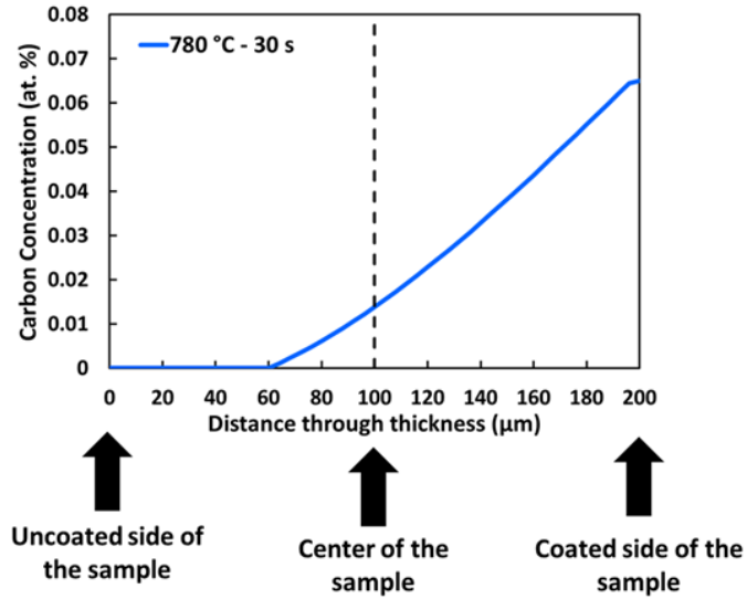
Fig. 6. Carbon distribution predicted theoretically using second Fick's diffusion law for heating at 780 °C for 30 seconds on a one-side coated specimen.
