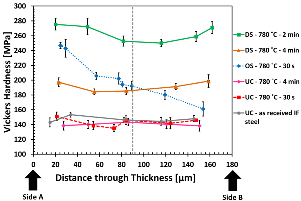
Fig. 3. Vickers microhardness through thickness for uncoated (UC) as received IF steel, one-side coated (OS) and double sides coated (DS) IF steel after induction heating at different temperatures and times. Side A indicates one side of the sample and side B is the other side of the tensile coupon. The dashed line at the center of the graph indicates the thickness center. For the one-side coated coupon (OS), side A is coated, while side B is without coating. Black error bars represent the standard deviation (print in color).
