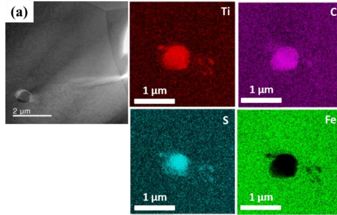
Fig. 16. BF-STEM image obtained from a coarse precipitate found in induction heated IF double side coated steel samples (a). According to EDS composition maps, this precipitate contains titanium, sulphur and carbon.
