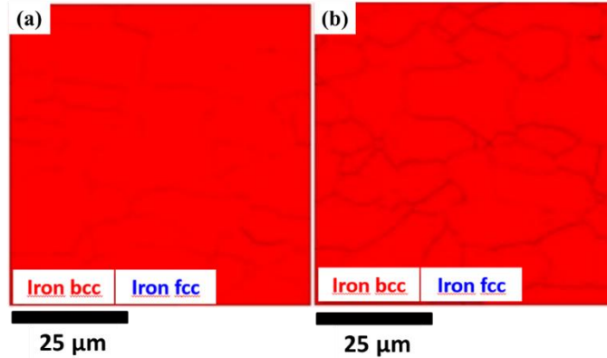
Fig. A. 1. Phase maps obtained from EBSD for specimens induction heated at 780 °C for 2 minutes (a) and 4 minutes (b).
