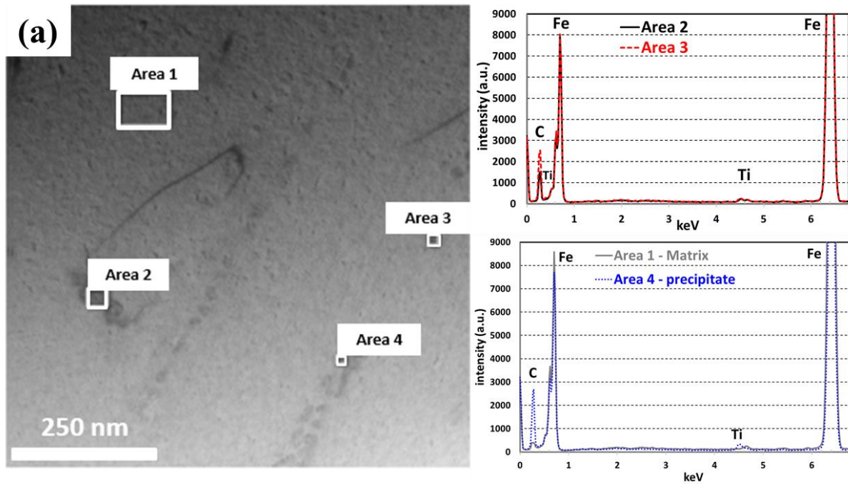
Fig. 14. BF-STEM image of the sample induction heated at 780 °C for 4 minutes showing in dark contrast lattice distortions created by dislocations and nanoscaled carbides (a). Locations of EDS spectra (1, 2, 3 and 4) are indicated in the image. Area 1 is obtained from the matrix, while Area 2, 3 and 4 show measurements obtained from nanoscaled precipitates.
