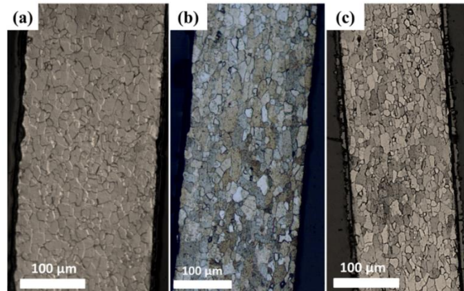
Fig. 8. Optical microscope images of thickness cross section for: uncoated and as received IF (a), uncoated IF induction heated at 780 °C for 2 minutes (b), uncoated IF induction heated at 780 °C for 4 minutes (c).
