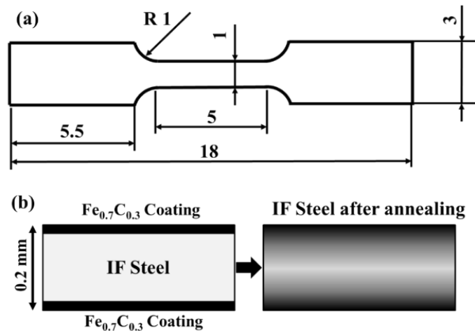
Fig. 1. (a) Dog-bone tensile sample (all dimensions are in mm), (b) schematic view of the thickness for IF steel double side coated before and after annealing.
