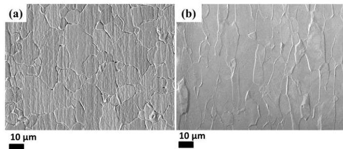
Fig. 10. Scanning Electron Microscope images of thickness cross section for: double side coated IF steel induction heated at 780 °C – 2 minutes (a) and double side coated IF steel induction heated at 780 °C for 4 minutes (b).
