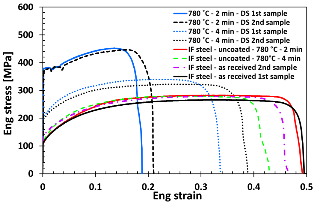
Fig. 7. Engineering stress-strain curves for coupons of IF steel coated double sides (DS) with 500 nm thick FeC film and induction heated for 2 and 4 minutes. Engineering stress-strain curves of uncoated and as received IF steel and of uncoated but induction heated specimens are included (print in color).
