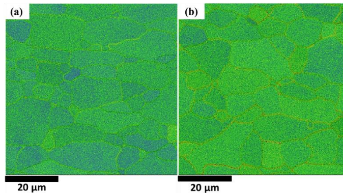
Fig. A. 2. Local misorientation and band contrast maps obtained from EBSD for specimens induction heated at 780 °C for 2 minutes (a) and 4 minutes (b).
