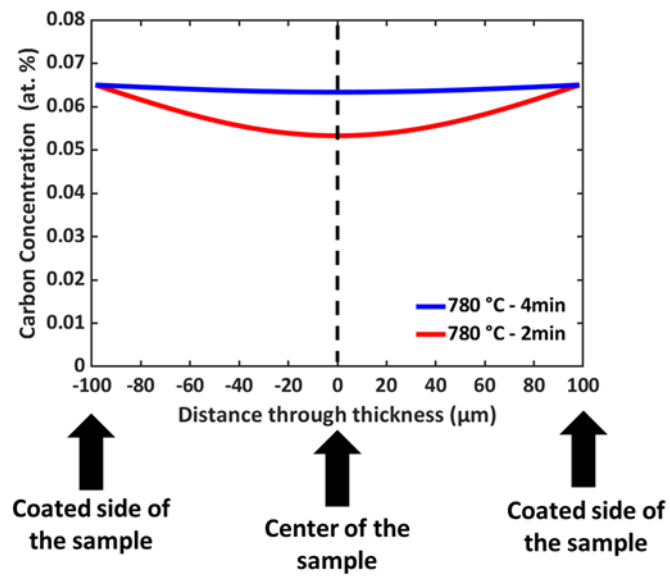
Fig. 5. Carbon distribution predicted theoretically using second Fick's diffusion law for heating at 780 °C for 2 minutes and 4 minutes on a double side coated specimen.
