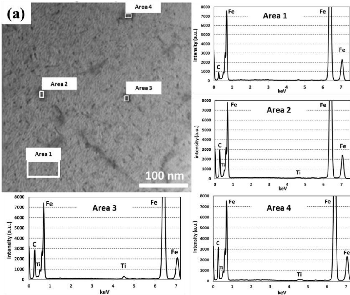
Fig. 13. BF-STEM image of the sample induction heated at 780 °C during 2 minutes showing in dark contrast lattice distortions created by dislocations and nanoscaled carbides (a). Locations of EDS spectra (1, 2, 3, 4) are indicated in the image. Area 1 is the reference taken in the matrix where Ti is below the detection limit. Area 2, 3 and 4 clearly exhibit the Ti-K peak, confirming the presence of nanoscaled TiC carbides.
