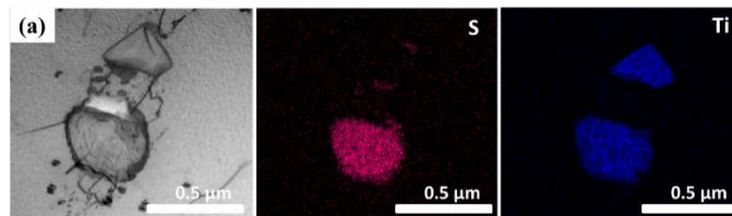
Fig. 15. BF-STEM image from a micron-sized precipitate found in induction heated IF double side coated steel samples (a). EDS composition maps show that it contains titanium and sulphur.
