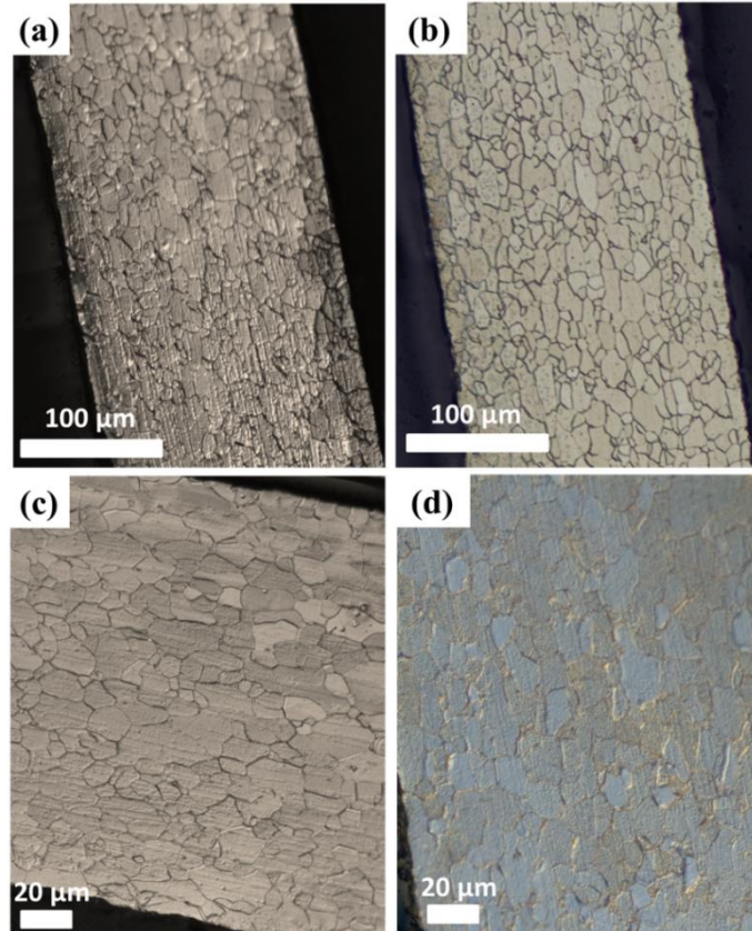
Fig. 9. Optical microscope images of thickness cross section for: both sides coated IF steel induction heated at 780 °C – 2 minutes (a) and (c), both sides coated IF steel induction heated at 780 °C for 4 minutes (b) and (d).
