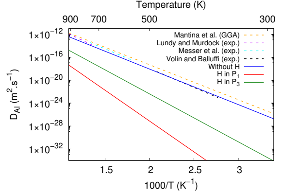
Figure 8: Calculated self-diffusion coefficient for Al, including previous work of Mantina et al [63], Lundy and Murdock [69], Messer et al [71], Volin and Balluffi [70]
