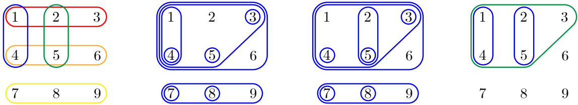
Figure 1: The elementary blocks of a building set \mathcal{B}_\circ (left), the two adjacent maximal \mathcal{B}_\circ -nested sets \mathcal{N}_\circ and \mathcal{N}'_\circ (middle), and the corresponding exchange frame (right).
