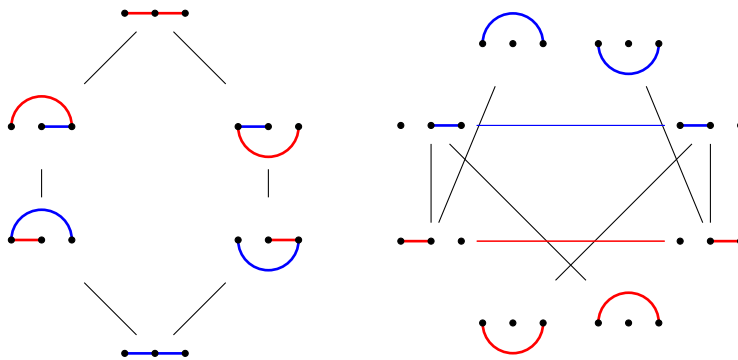
Figure 5: The weak order on \mathfrak{S}_3 with permutations labeled by semi-crossing arc biduals, and the canonical complex of \mathfrak{S}_3 with join and meet irreducible permutations labeled by arcs.
