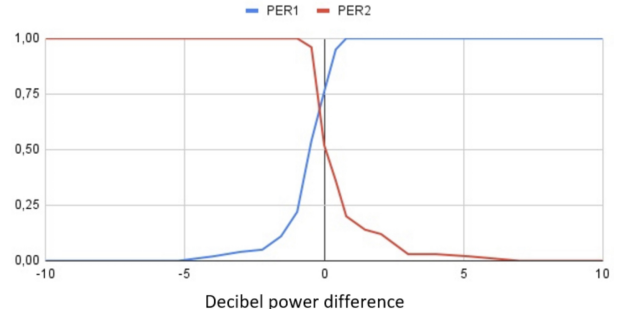
Fig. 3: Capture effect and Packet Error Rate (PER) for both transmitters.
