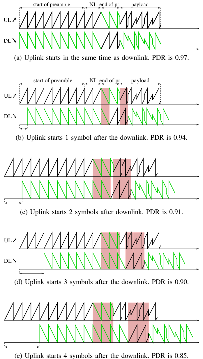
Fig. 1: Concurrent uplink and downlink transmissions as a function of the time offset between the two frames. The red boxes represent collisions between upchirps (in black) and respectively downchirps (in green) from different frames. The PDR is computed as the mean between uplink and downlink PDRs in the specified setup.
