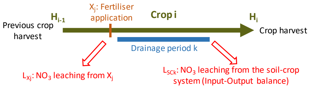
Fig. 2. Generic representation of surface leaching from N inputs ( L_{Xj} ) and profile leaching from the soil-crop system ( L_{Sck} ) for the draining period k , for crop i , between the harvest of the previous crop ( H_{i-1} ) and the crop harvest
