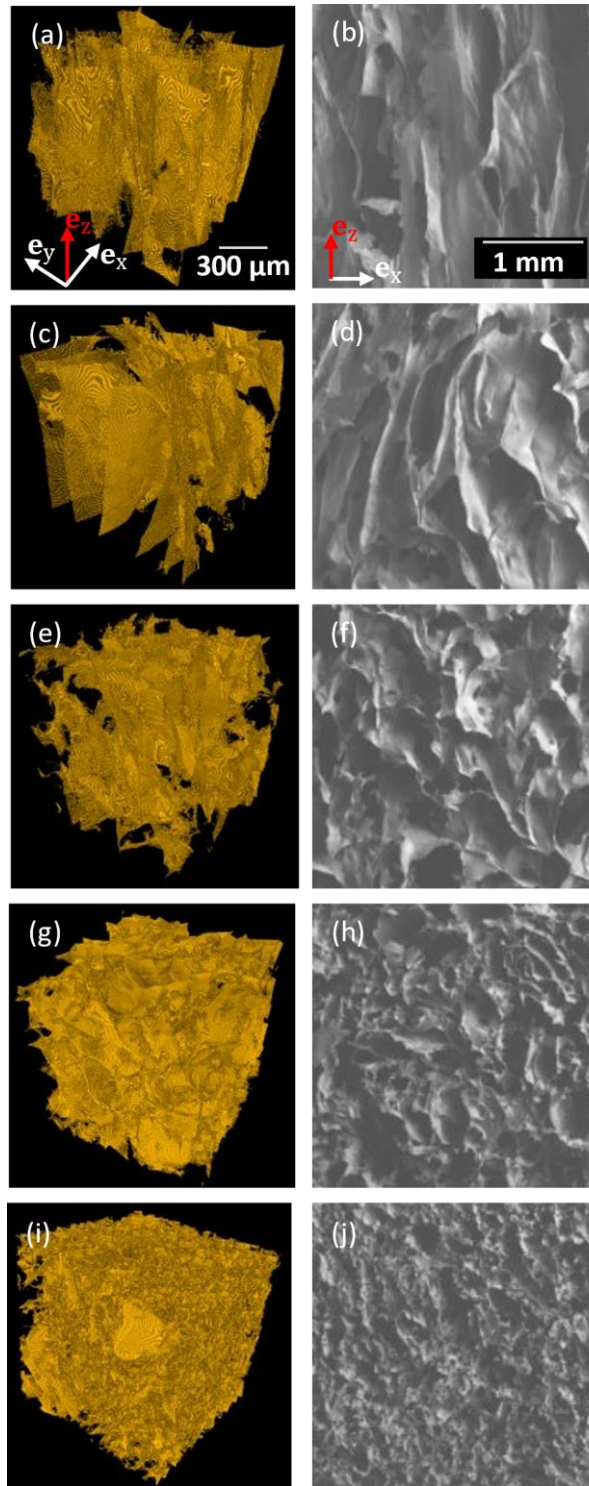
Figure 6. 3D (X-Ray nanotomography) (left) and 2D (SEM) micrographs (right) showing the structures of CNF foams along the freezing direction \mathbf{e}_z within Zone 2 at various studied relative densities \rho/\rho_s : 0.003 (a, b), 0.0063 (c, d), 0.01 (e, f), 0.05 (g, h) and 0.079 (i, j).
