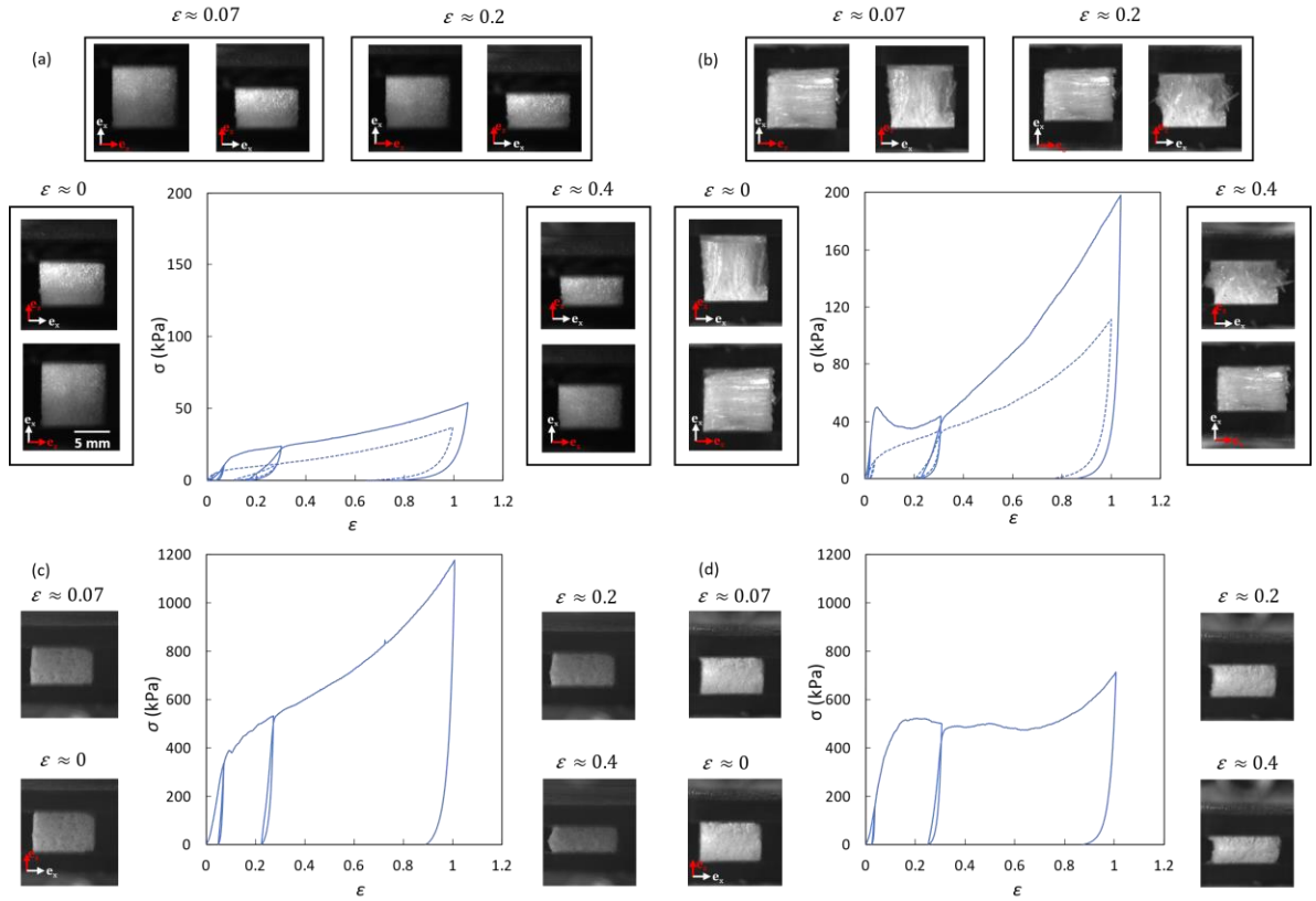
Figure 11. Typical stress-strain curves for CNF (a, with \rho/\rho_s \approx 0.01 and c, with \rho/\rho_s \approx 0.078 ) and CNC foams (b, with \rho/\rho_s \approx 0.052 and d, with \rho/\rho_s \approx 0.135 ). The photographs show deformed samples at various strains. At standard relative densities (a,b), as the foams exhibited anisotropic properties, the graphs show the compression responses along the freezing direction \mathbf{e}_z (solid line) and perpendicular to it (dashed line) with corresponding photographs of the samples at various strains.
