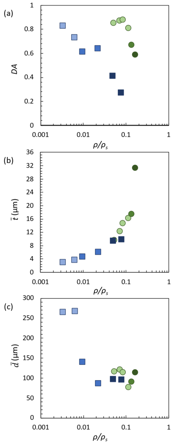
Figure 10. Evolutions with the relative density \rho/\rho_s of the degree of anisotropy DA (a), the mean cell wall thickness \bar{t} (b) and the mean pore thickness \bar{d} for TEMPO-oxidised CNF foams (square symbols) and CNC foams (circular symbols). The differences in the shades represent the transitions in the pore microstructures, from columnar/lamellar pores (light colours) to more isotropic pores (darker colours).
