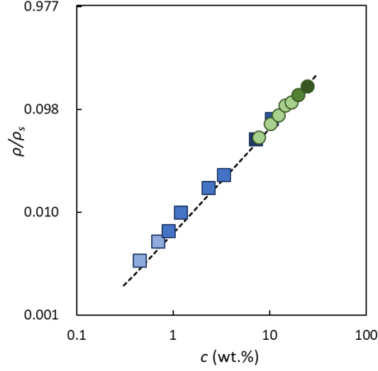
Figure 4. Evolution of the measured relative density \rho/\rho_s of CNF (square symbols) and CNC foams (circular symbols) with the hydrogel concentration c . The dashed line is the theoretical value \rho_t/\rho_s given by Eq. (1). The differences in the shades represent the transition in the pore microstructures from columnar/lamellar pores (light colours) to more isotropic pores (darker colours).
