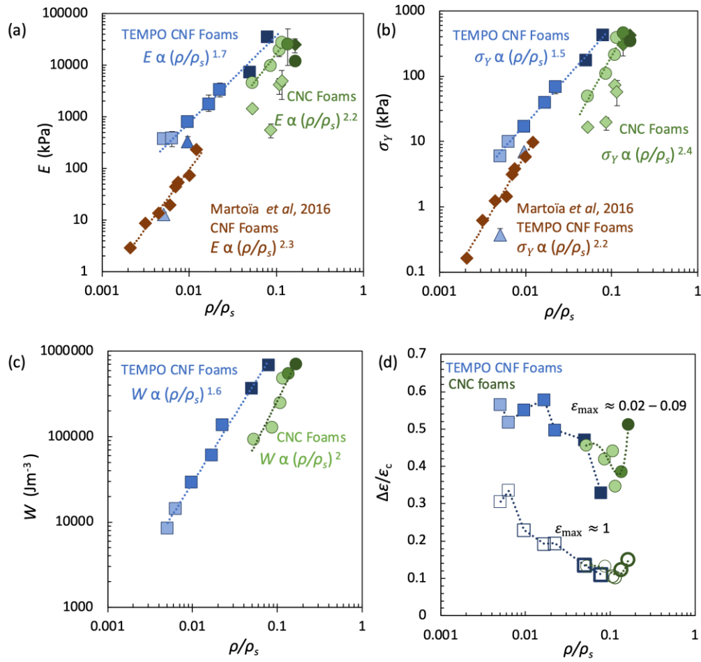
Figure 12. Evolutions with the relative density \rho/\rho_s of the CNC (green circular symbols) or CNF (blue square symbols) Young's moduli E (a), yield stress \sigma_y (b), absorbed energy per unit volume W (c) and strain recovery ratio \Delta\epsilon/\epsilon_c (d). Squares or circles and triangles or diamonds are the data obtained in directions parallel and perpendicular to the freezing direction, respectively. Graphs (a) and (b) also show the data obtained by Martoia et al. [11] for TEMPO-oxidised foams with radial (anisotropic) ice-templating. The difference in the shades represents the transitions in the pore microstructures, from columnar/lamellar pores (light colours) to more isotropic pores (darker colours).
