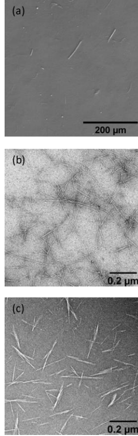
Figure 1. Micrographs showing (a) remaining partially fibrillated wood fibers in the TEMPO-oxidised CNF hydrogels (SEM), TEMPO-oxidised CNFs (TEM), (c) hydrolysed CNCs.
