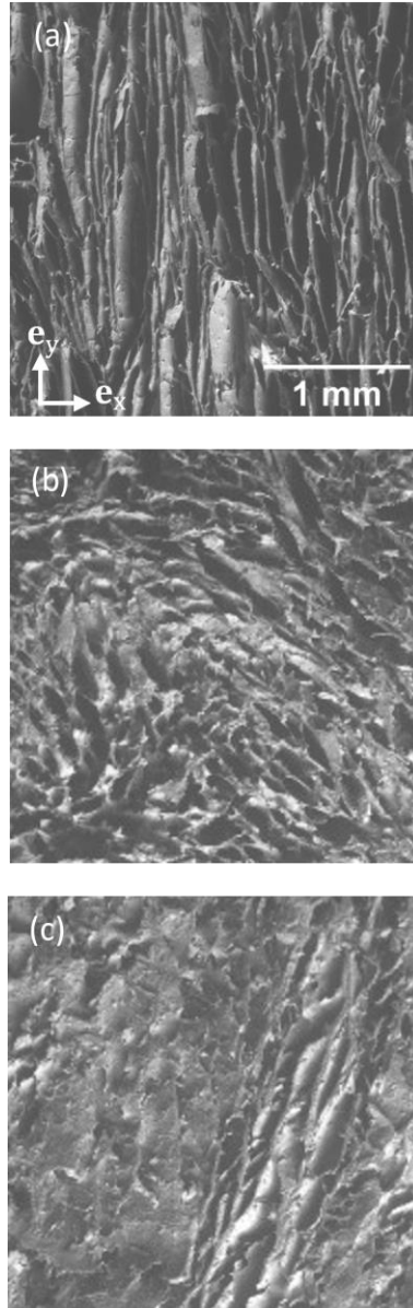
Figure 9. SEM micrographs showing the microstructures of CNC foams perpendicular to the freezing direction \mathbf{e}_z in Zone 2 at various relative densities \rho/\rho_s = 0.108 (a), 0.135 (b) and 0.164 (c).
