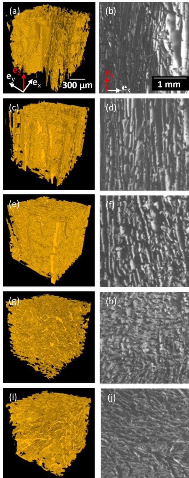
Figure 8. 3D (X-Ray nanotomography) (left) and 2D (SEM) micrographs (right) showing the structures of CNC foams along the freezing direction \mathbf{e}_z within Zone 2 at various relative densities \rho/\rho_s = 0.052 (a, b), 0.086 (c, d), 0.115 (e, f), 0.135 (g, h) and 0.164 (i, j).
