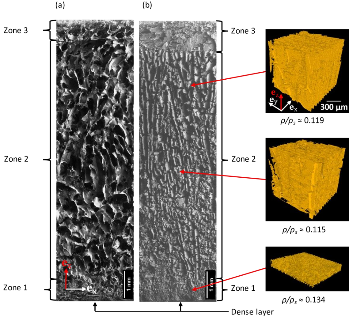
Figure 5. SEM micrographs of a CNF foam ( \rho/\rho_s = 0.01 ) (a) and CNC foam ( \rho/\rho_s = 0.115 ) (b), showing sections along the freezing direction \mathbf{e}_z with the three different zones 1, 2 and 3 induced during ice-templating. The red arrows indicate where the 3D images (on the right, X-Ray nanotomography) of CNC foams were acquired.
