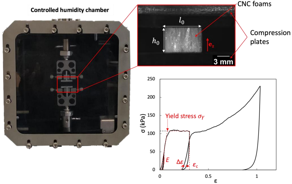
Figure 3. Compression experimental setup installed in the controlled humidity chamber and mounted on the electromechanical tension-compression machine. The zoom shows a CNC foam sample ( \rho/\rho_s \approx 0.086 ) placed between the compression platens before compression along the freezing direction e_z . Below is plotted the corresponding stress-strain curve.
