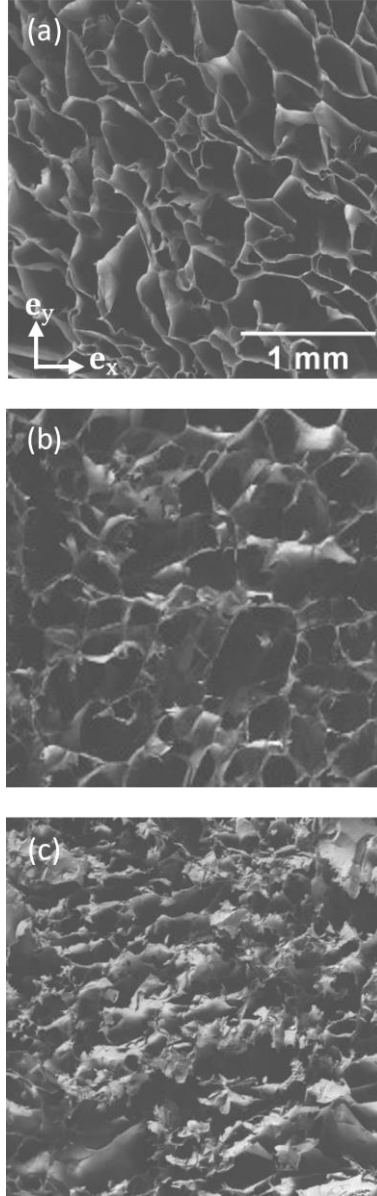
Figure 7. SEM micrographs showing the structures of CNF foams perpendicular to the freezing direction \mathbf{e}_z within Zone 2 at various relative densities \rho/\rho_s = 0.003 (a), 0.01 (b) and 0.05 (c).
