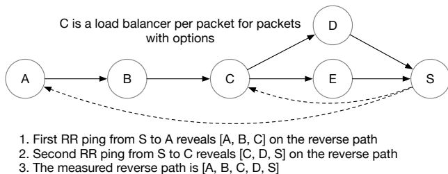
Figure 10: Reverse Traceroute reveals one accurate reverse path in presence of load balancing.
