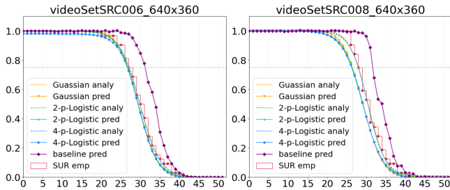
Fig. 4: Examples of SUR prediction results comparison between SRC-based models and baseline model
