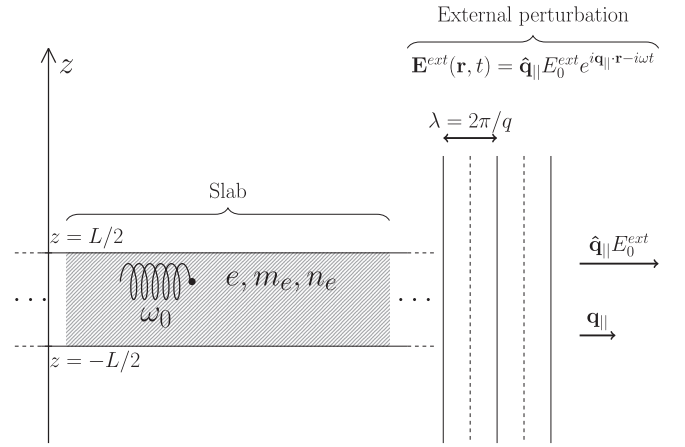
FIG. 6. Slab undergoing an external longitudinal perturbation of wave vector \mathbf{q} and frequency \omega , with the electric field parallel to the surface.
