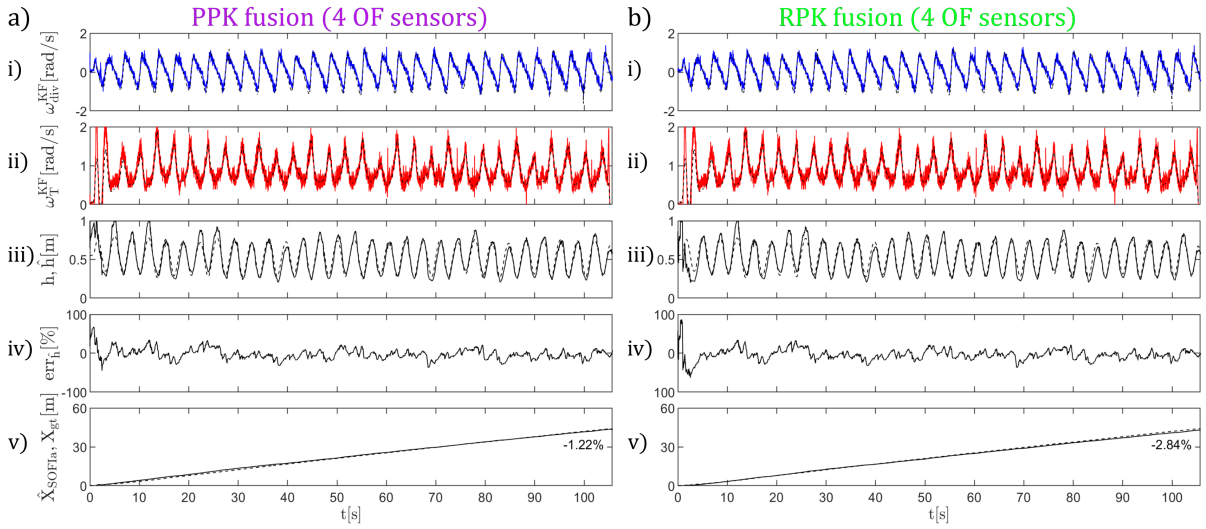
Figure 6: The local Optic Flow (OF) divergence \omega_{div}^{KF} (in blue) measured with the Precise Prior Knowledge (PPK) strategy had a Signal-to-noise Ratio (SnR) of 6.72dB (a.i) and with the Rough Prior Knowledge (RPK) strategy of 6.73dB (b.i). The theoretical local optic flow divergence was computed as the ratio between V_h and h (in dashed line). The local translational optic flow \omega_T^{KF} (in red) measured with the PPK strategy had a SnR of 25.74dB (a.ii) and with the RPK strategy of 25.91dB (b.ii). The theoretical local translational optic flow was computed as the ratio between V_x and h (in dashed line). The estimates of the flight height \hat{h} converged quickly (within 4s) to the ground truth h in both cases (a and b.iii). The average percentage error of \hat{h} with respect to h after convergence was -2.16\% for the PPK strategy (with a range of [-36.89\%, 34.13\%] ) (a.iv) and -2.58\% for the RPK strategy (with a range of [-36.89\%, 34.23\%] ) (b.iv). The final percentage error in the estimates of the distance traveled \hat{X}_{SOFIa} with respect to the ground truth X_{gt} was -1.22\% for the PPK strategy (a.v) and -2.84\% for the RPK strategy (b.v).
