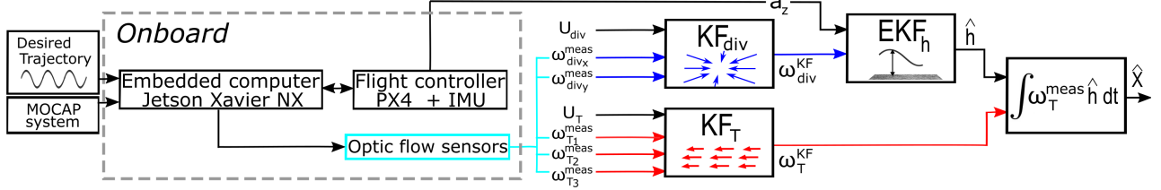
Fig. 3: The sensor fusion based on 4 optic flow sensors rely on additional Kalman Filters (KF). The embedded computer handles the 4 optic flow sensors set on the hexarotor. \omega_{div_x}^{meas} and \omega_{div_y}^{meas} are taken as measurements by a KF (noted KF_{div} ), that takes as input the current value U_{div} of the model of the optic flow divergence. The output of the KF is the local optic flow divergence \omega_{div}^{KF} . \omega_{T_1}^{meas} , \omega_{T_2}^{meas} and \omega_{T_3}^{meas} are taken as measurements by a KF (noted KF_T ), that takes as input the current value U_T of the model of the translational optic flow. The output of the KF is the local translational optic flow \omega_T^{KF} . The EKF takes as input the hexarotor’s acceleration a_z and as measurement \omega_{div}^{KF} to estimate the current flight height \hat{h} . The EKF output \hat{h} scales \omega_T^{KF} , that is then integrated to perform odometry.
