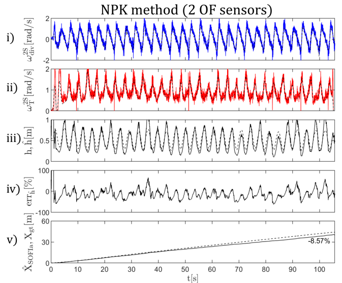
Fig. 5: i) The local Optic Flow (OF) divergence \omega_{div}^{2S} (in blue) measured with the No Prior Knowledge (NPK) method had a Signal-to-noise Ratio (SnR) of 5.62dB . The theoretical local optic flow divergence was computed as the ratio between V_h and h (in dashed line). ii) The local translational optic flow \omega_T^{2S} (in red) measured with the NPK method had a SnR of 19.12dB . The theoretical local translational optic flow was computed as the ratio between V_x and h (in dashed line). iii) The estimates of the flight height \hat{h} converged quickly (within 4s) to the ground truth h . iv) The average percentage error of \hat{h} with respect to h after convergence was -9.77\% (with a range of [-61.5\%, 65.34\%] ). v) The final percentage error in the estimates of the distance traveled \hat{X}_{SOFla} with respect to the ground truth X_{gt} was -8.57\% .
