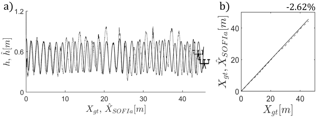
Fig. 7: a) Comparison of the position of the hexarotor in the vertical plane ( x,z ) estimated with the Rough Prior Knowledge (RPK) fusion strategy (dashed line) to the ground truth given by the MoCap system (continuous line). The estimates of the flight height \hat{h} were plotted on the estimates of the traveled distance \hat{X}_{SOFIa} , while the ground truth h was plotted on X_{gt} . This test flight was performed at 1518lux . b) The final percentage error in the estimates of the traveled distance \hat{X}_{SOFIa} with respect to the ground truth X_{gt} was -2.62\% .
