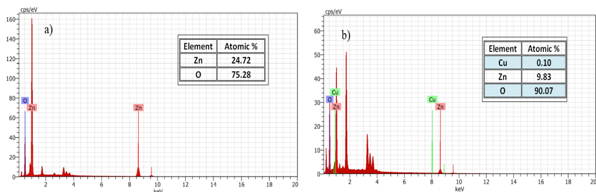
Fig. 2. EDS spectrum obtained for: a) ZnO, b) Cu-doped ZnO.
