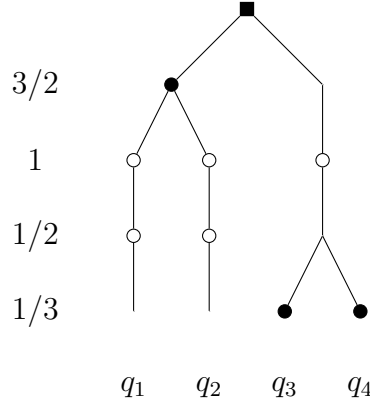
FIGURE 1. The fission tree \mathcal{T}^p associated to Q (not drawn isometrically). The labelling corresponds to the numbering of the q_i . The multiplicities of the leaves are all equal to 1.
