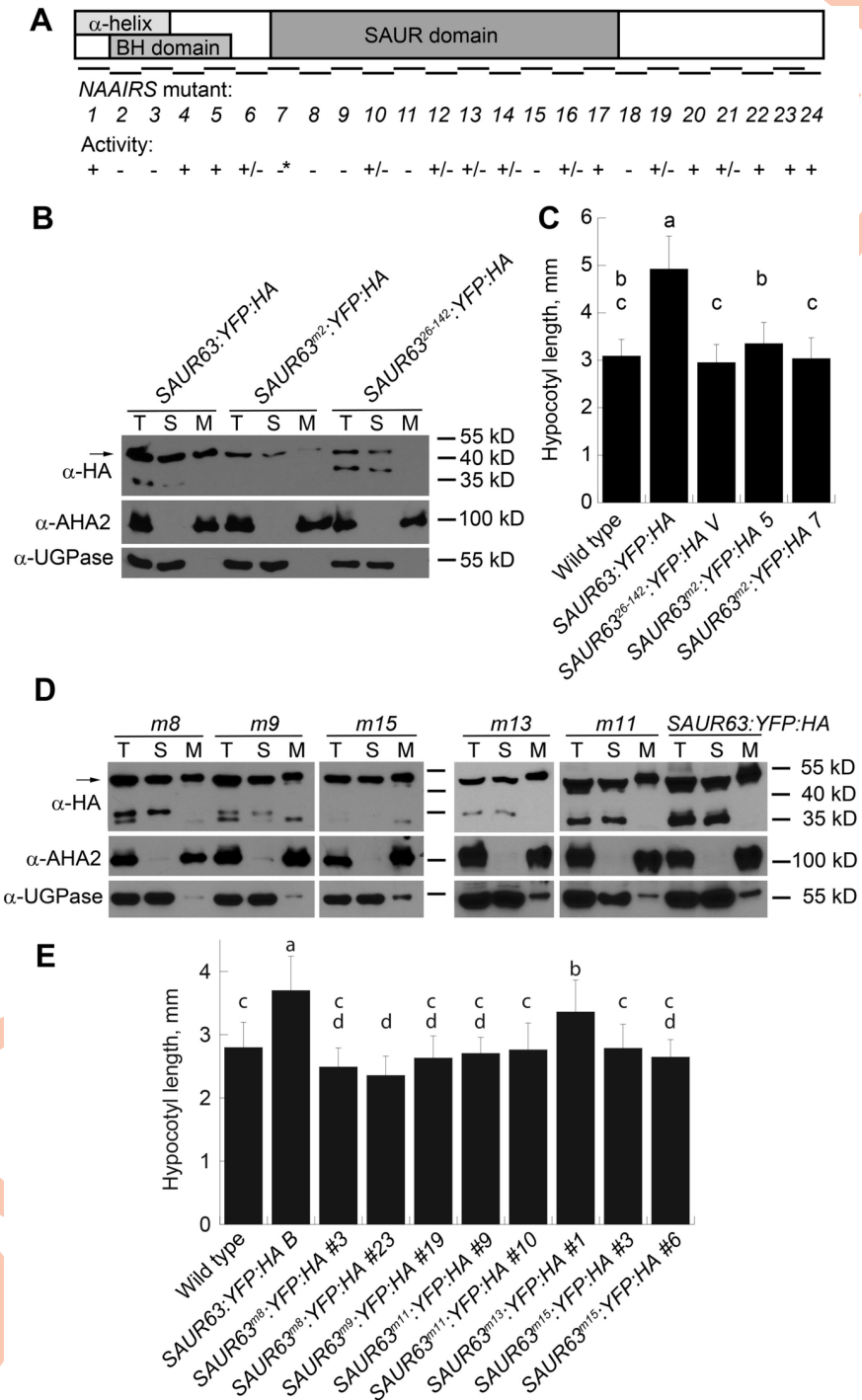
Fig 7. Effects of mutations on SAUR63 properties. A) Diagram of SAUR63 indicating predicted structural features, locations of NAAIRS mutations m1-m24 , and whether SAUR63:YFP:HA and/or SAUR63YFP:HA fusion proteins with each mutation retained function, based on their ability to confer either tortuous root growth or increased hypocotyl elongation in Figs 7C and 7E and S11 and S1 Table. +, caused phenotypes in all experiments; -, failed to cause phenotypes in all experiments; +/- caused phenotypes in at least one experiment; *, no fusion protein detected. B,D) Fusion proteins in stable P 35S :SAUR63 NAAIRS :YFP:HA lines, detected by western blots in total (T), soluble (S) and microsomal (M) protein fractions. \alpha -HA detects SAUR63:YFP:HA fusion protein variants; \alpha -AHA2 detects a membrane protein; \alpha -UGPase detects soluble proteins. In D, P 35S :SAUR63 NAAIRS :YFP:HA line names are abbreviated by the mutation name ( m8 etc.). C,E) Hypocotyl lengths of stable lines of seedlings grown for 4d in short days. Graph shows means \pm s.d. Letters indicate statistical classes based on Tukey's Honestly Significant Difference test. n, from left to right: panel C: 55, 30, 34, 31, 36; panel E: 17, 24, 29, 21, 24, 27, 29, 24, 29, 30.
