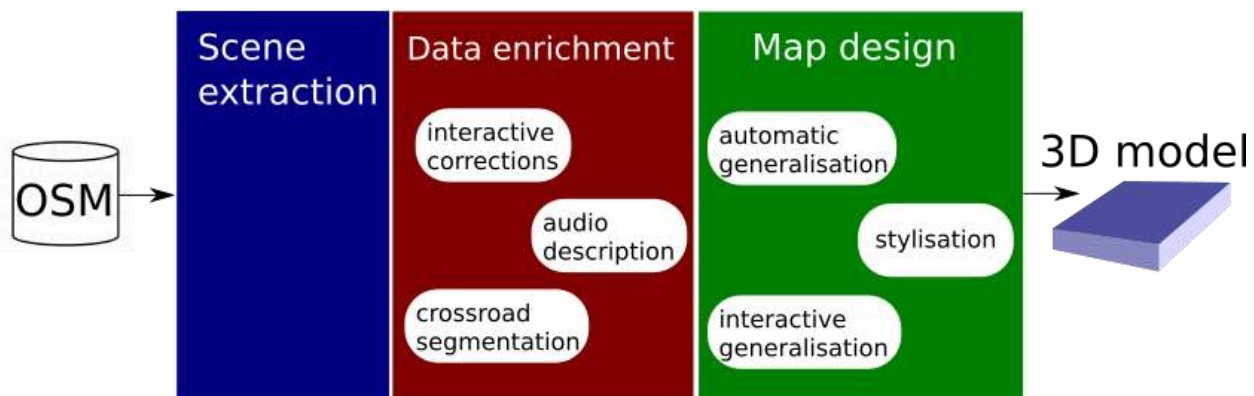
Figure 1. Functionalities of the MULTIMAGE platform to generate a 3D model for a tactile from OpenStreetMap data: (1) a scene (a crossroad for now) is extracted; (2) the OSM data is enriched and corrected with a mix of automated scripts and interactive actions; (3) the map is designed with the enriched data with a mix of automated scripts and interactive actions.
