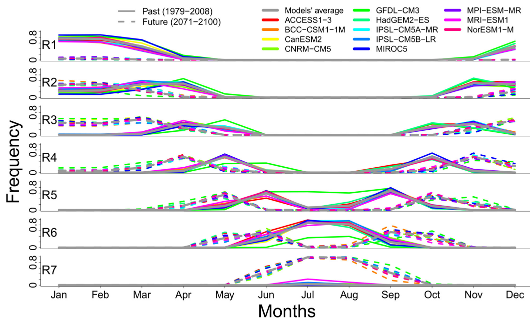
FIGURE 6 Average annual cycle of the seven regimes for the 12 climate models in the past (1979–2008) and future (2071–2100) [Colour figure can be viewed at wileyonlinelibrary.com ]
