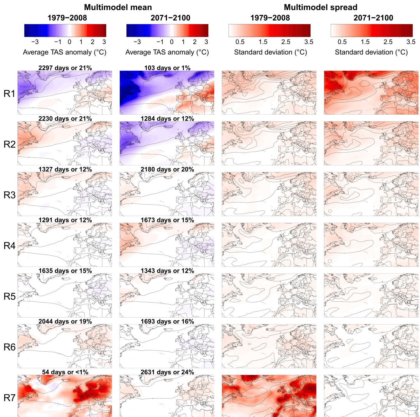
FIGURE 5 As in Figure 4 but for TAS anomalies conditionally to the regimes [Colour figure can be viewed at wileyonlinelibrary.com ]
