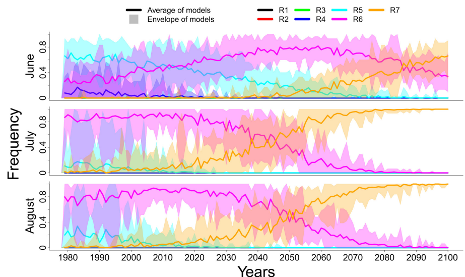
FIGURE 8 As in Figure 7 but for June, July and August [Colour figure can be viewed at wileyonlinelibrary.com ]
