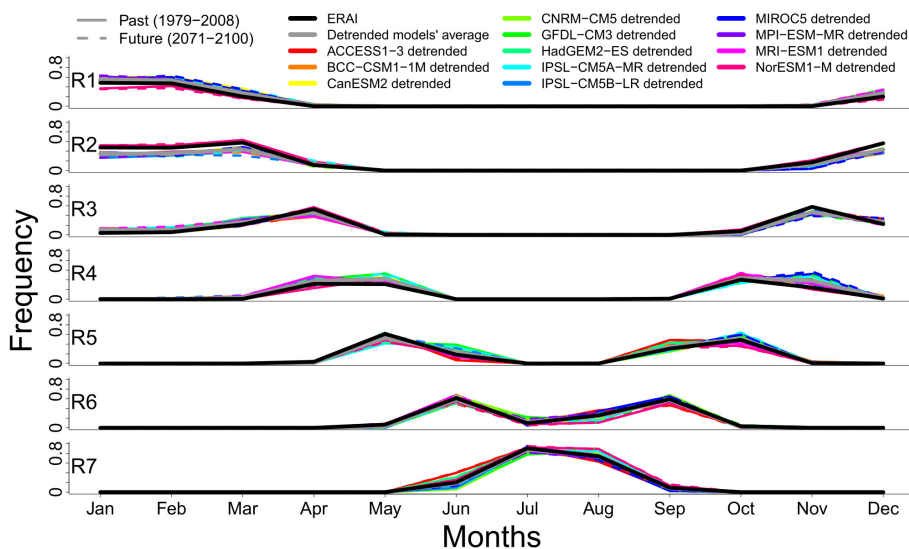
FIGURE 9 As in Figure 6 but after detrending the data from climate models [Colour figure can be viewed at wileyonlinelibrary.com ]
