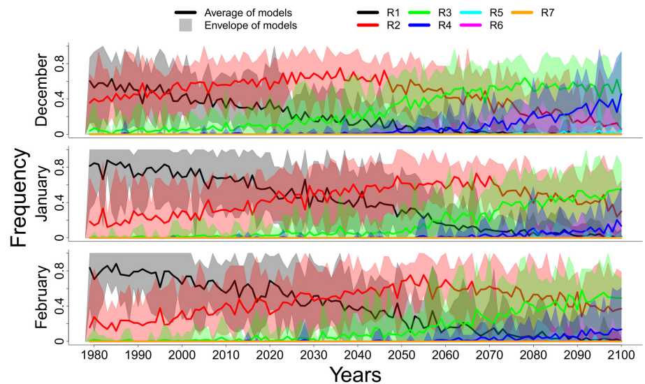
FIGURE 7 Frequency of the regimes per year in December, January and February for the 12 climate models [Colour figure can be viewed at wileyonlinelibrary.com ]
