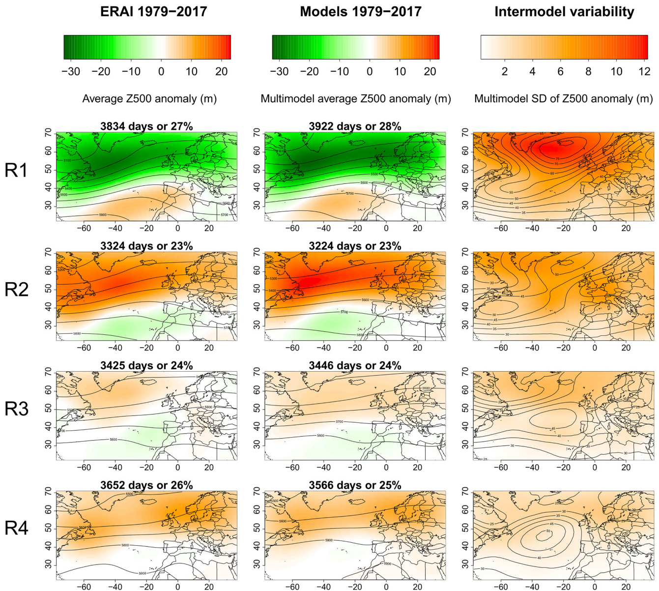
FIGURE 1 Composite maps of the four regimes (one per row) for ERAI (first column) and climate models (second column; each map shows the average of 12 composite maps; third column shows standard deviation of Z500 between the 12 composites). The maps are calculated by averaging the seasonal anomalies (shading) and raw values (contour lines) over the days belonging to the regime. Seasonal anomalies correspond to the raw values minus the average seasonal cycle. The number of days per regime is shown above each map (average of 12 values for the climate models) [Colour figure can be viewed at wileyonlinelibrary.com ]
