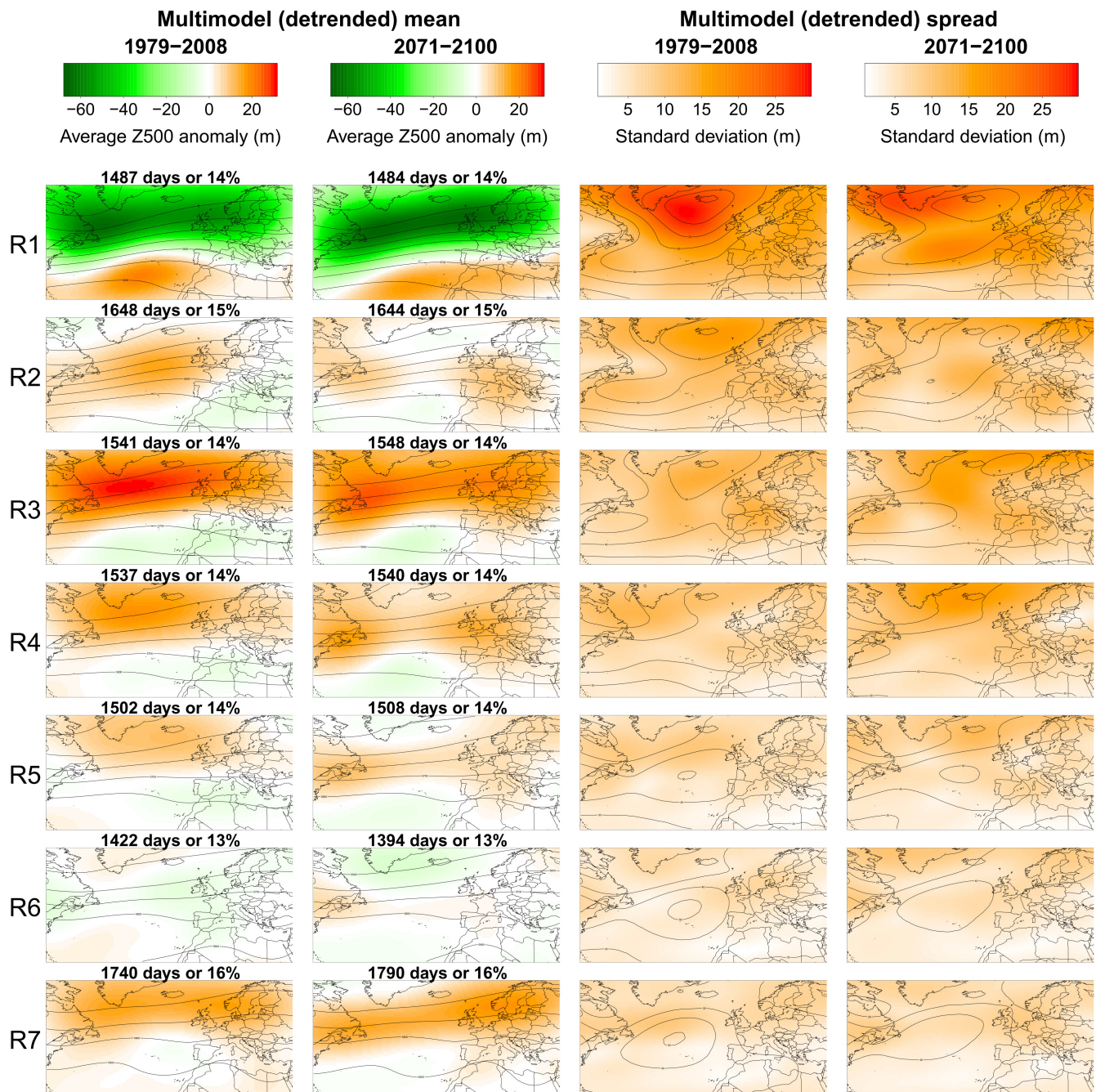
FIGURE 10 As in Figure 4 but after detrending the data from climate models [Colour figure can be viewed at wileyonlinelibrary.com ]
