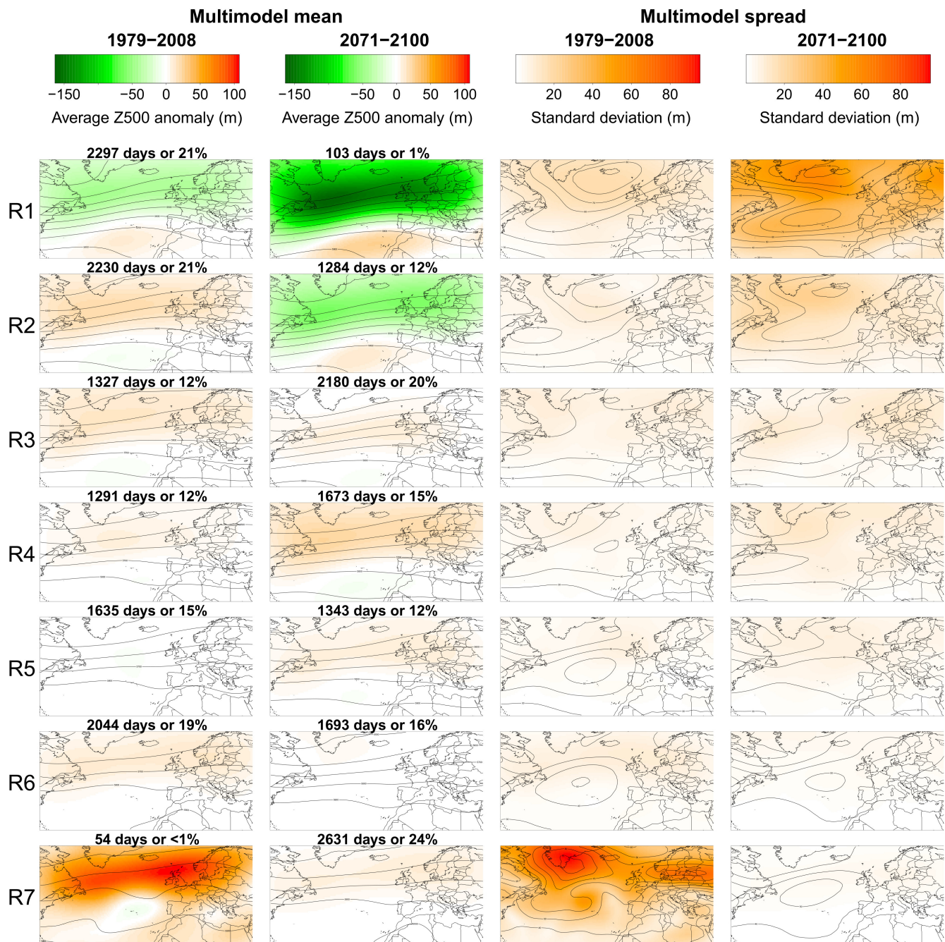
FIGURE 4 Same as Figure 1 but for the climate models (without ERAI) and seven regimes over 1979–2100. The seasonal anomalies are calculated with reference to the average seasonal cycle of the subperiod (1979–2008, 2071–2100) [Colour figure can be viewed at wileyonlinelibrary.com ]
