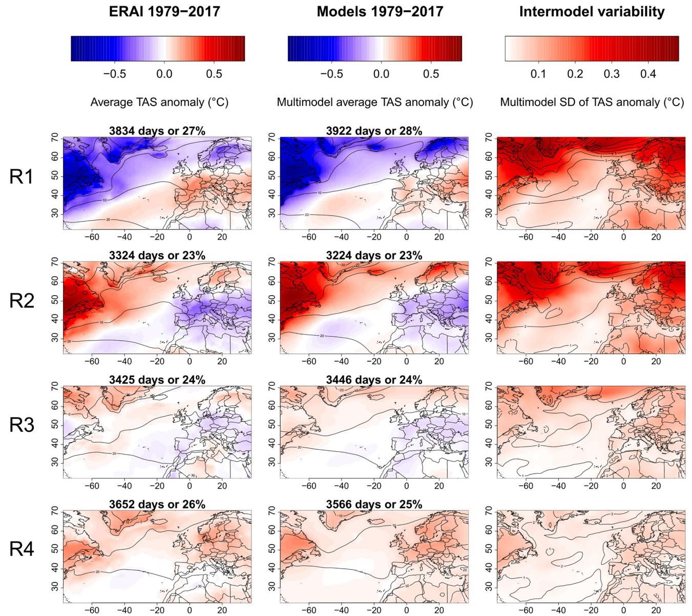
FIGURE 3 As in Figure 1 but for TAS conditionally to each regime [Colour figure can be viewed at wileyonlinelibrary.com ]
