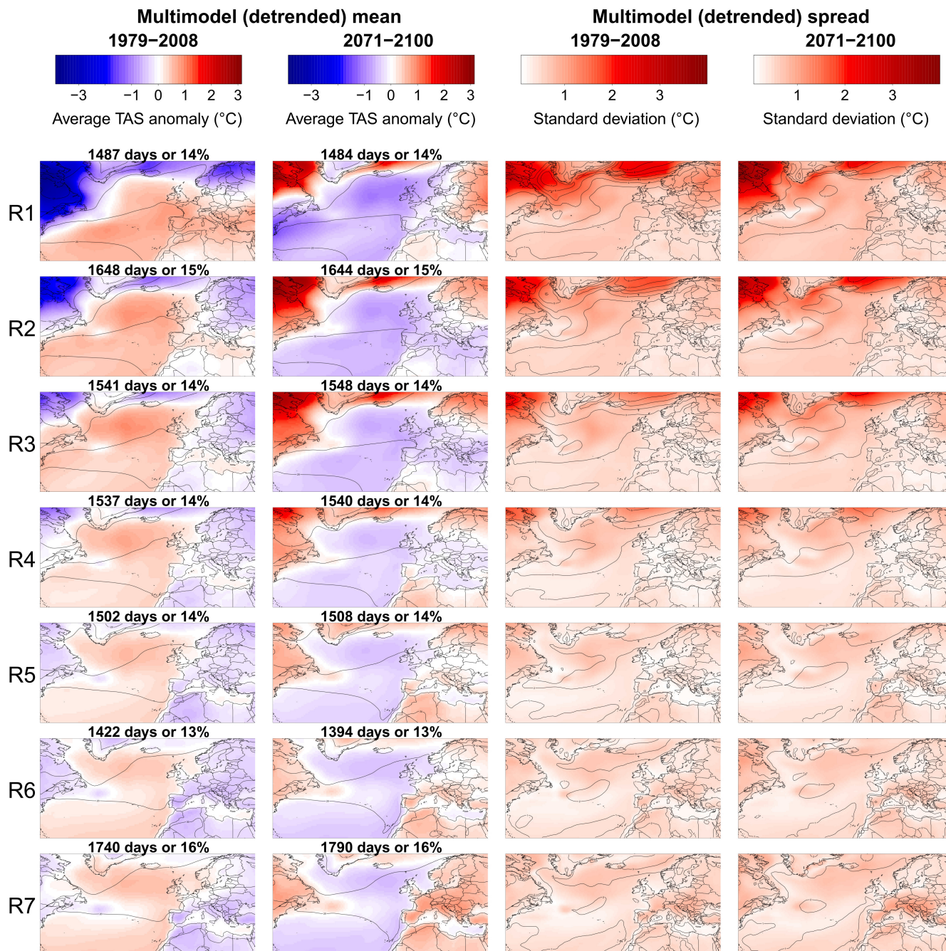
FIGURE 11 As in Figure 5 but after detrending the data from climate models [Colour figure can be viewed at wileyonlinelibrary.com ]
