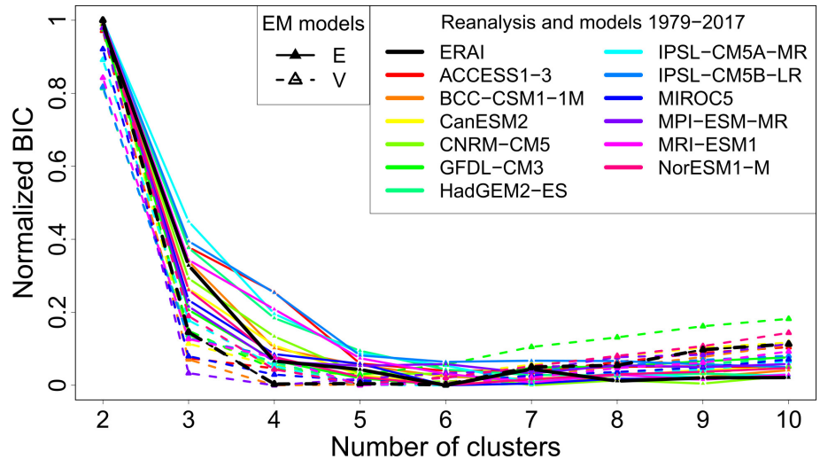
FIGURE A1 Bayesian information criterion (BIC) of the clustering models in function of the number of clusters and model type for ERAI and each climate model over 1979–2017 (exception of HadGEM2-ES: 1981–2017). The BIC values are normalized between 0 (best EM model) and 1 (worst EM model). E: equal variance, V: variable variance [Colour figure can be viewed at wileyonlinelibrary.com ]
