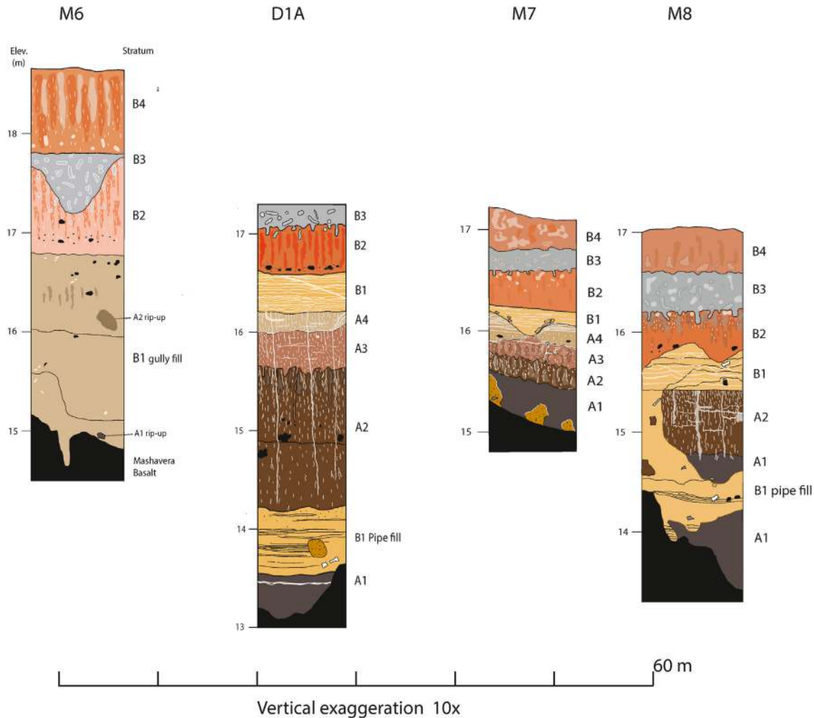
Figure 7. Section of profiles north of Blocks 1 and 2 showing gully and pipe features. These profiles illustrate the contexts and results of gully and piping on the upper promontory (see Fig. 1c for locations). The M6 primary gully provided a gully wall exit for sediments removed from the pipe in D1A. The fully exposed pipe adjacent to D1A was filled with B1 sediment, with numerous bones in the lower pipe fill. Note that B1 slope facies surmount Stratum A deposits here. High basalt in M7 resulted in thinner Stratum A deposits and sheetwash toward the lower promontory. The pipe in M8 was breached and then filled with B1 sediment with bones, stones, and rip-ups of Stratum A2 in the pipe fill. Note the erosion of B1 in the M8 profile, and the uniform burial of B1 deposits by B2–B4 in these four profiles. Abbreviation: Elev. = elevation.
