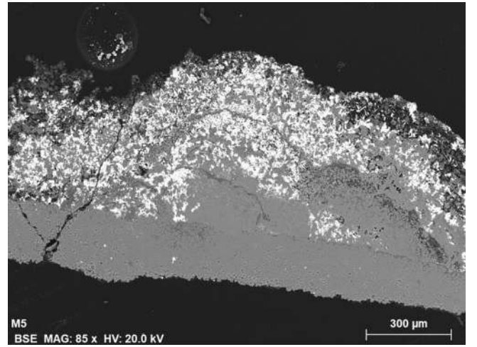
Fig. 9. BSE image of sample M5 showing the progressive replacement of the initial calcitic phase (dark phase) by celestine (white phase). The darker phase corresponds to high porosity calcite. SEM images have been acquired using a HIROX SH3000 microscope equipped with a KE BSE detector.
