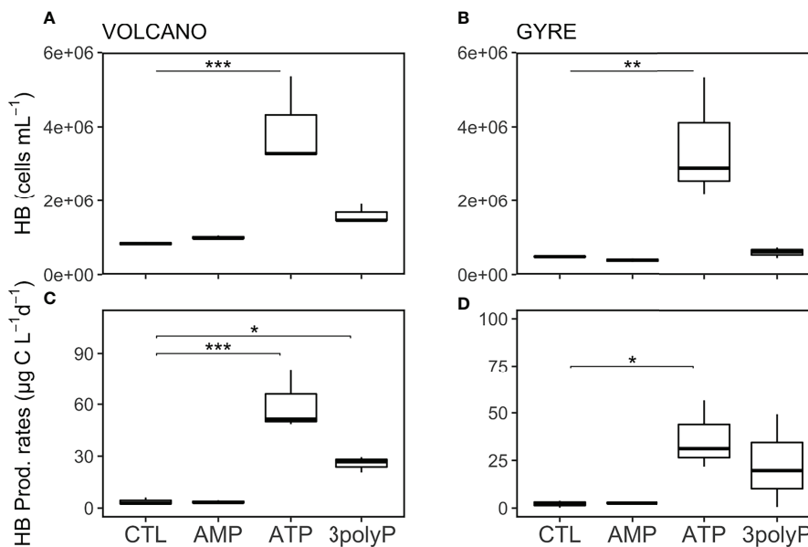
FIGURE 4 | Abundance and production rates of heterotrophic bacteria. Boxplots represent averaged heterotrophic bacteria (HB) abundance ( A, B ) and production rates ( C, D ) from each treatment triplicate at the volcano and the gyre station, respectively. Significant differences in cell abundance between the control and the DOP treatments were tested with the Dunnett's Test and represented by the horizontal lines with significance codes (** p < 0.001 , * p < 0.01 , * p < 0.1 ).
