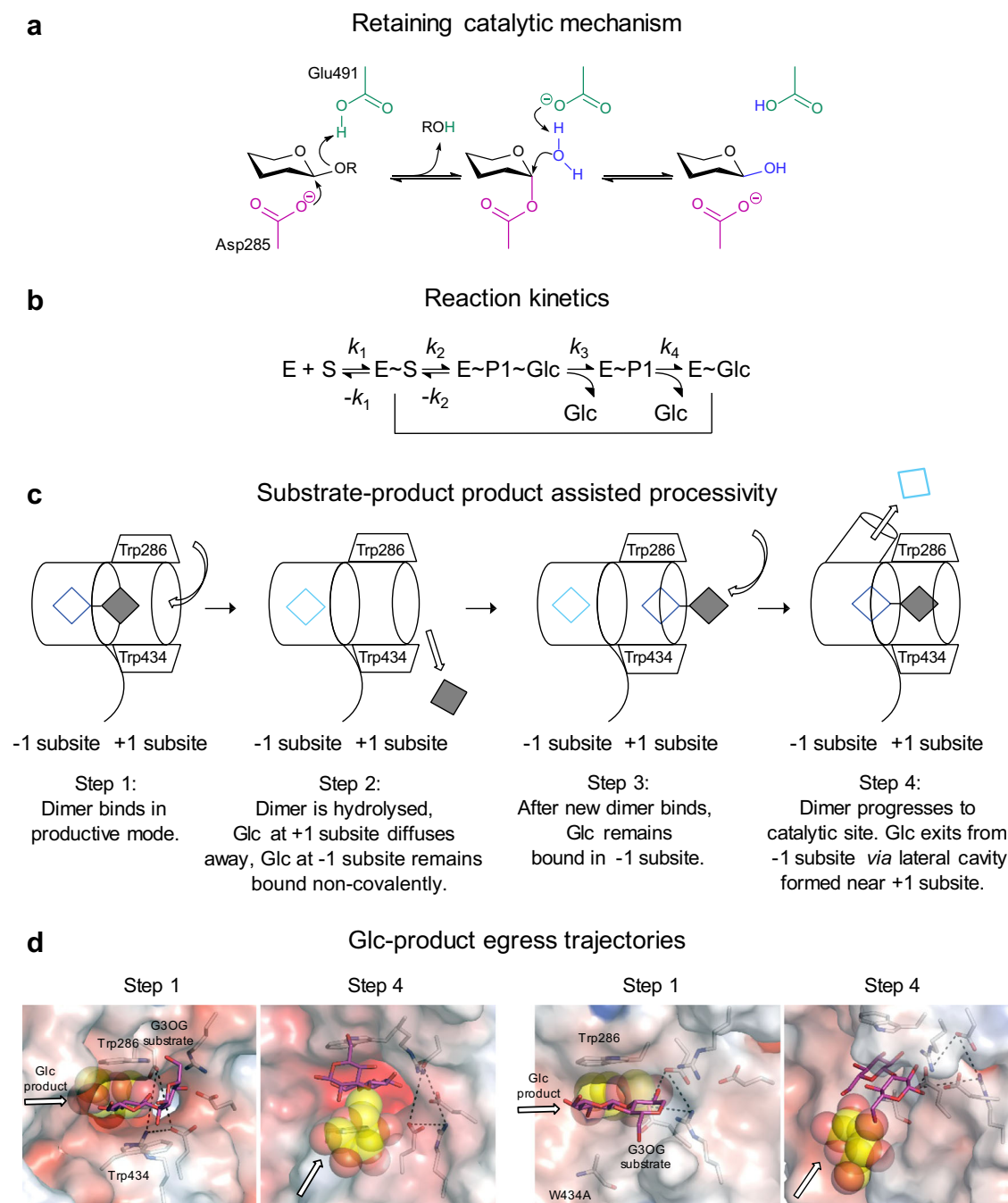
Fig. 9 | Mechanistic view of the catalytic function of HvExoI, a family GH3 enzyme. a HvExoI uses the retaining catalytic mechanism, where nucleophile Asp285 (magenta) and acid/base catalyst Glu491 (green) play key roles in substrate hydrolysis 1-3 . b Reaction kinetics indicates the formation of Michaelis complexes (E-S and E-S), and enzyme-product complexes before (E-P1-Glc) and following the first Glc egress (E-P1), and after hydrolysis of P1 (E-Glc) 1,2 . S and P1 are trimeric and dimeric molecules, respectively. First-order rate constants are shown. Entrapped Glc product from E-Glc is displaced after a new substrate is attached. The hydrolytic cycle with a (1,3)-linked substrate is repeated until it is hydrolysed to Glc (indicated by vertical and horizontal lines). c Simplified mechanism of Glc displacement with a disaccharide 22 . After the disaccharide (empty blue and filled grey
