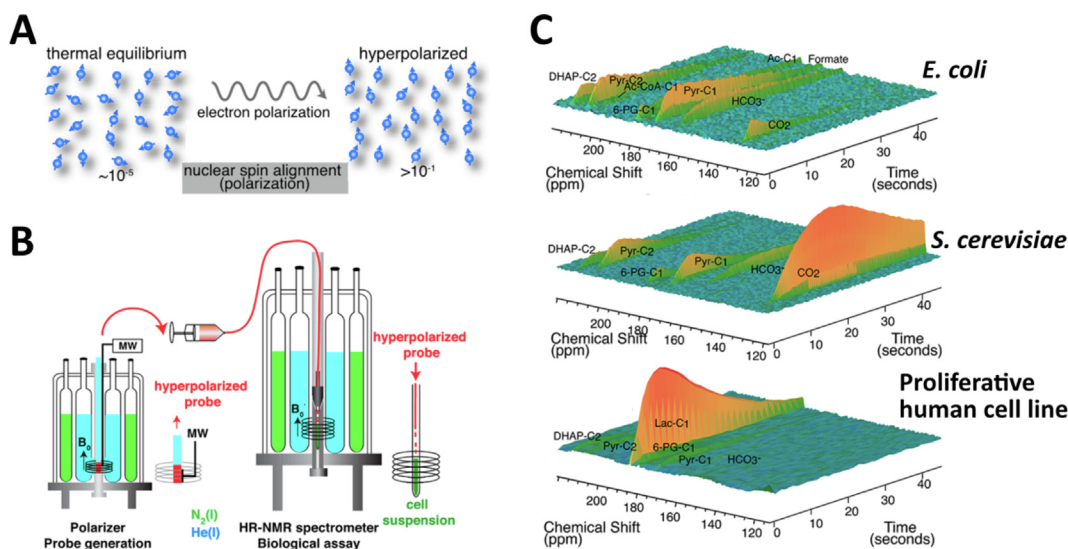
Fig. 18. A) Operating principle of Dynamic Nuclear Polarization (DNP). Current technologies in common use employ intense microwaves to polarize nuclear spins in the presence of polarizing agents (particular molecules containing unpaired electrons, i.e. free radicals) at cryogenic temperatures; B) Operating principle of dissolution-DNP: hyperpolarization of nuclear spins is reached at cryogenic temperature under microwave (MW) irradiation; the hyperpolarized substrate is then dissolved in the final liquid sample for analysis (here suspension cells); C) Stacked one-dimensional ^{13}\text{C} -NMR spectra showing real-time observation of glucose in E. coli , S. cerevisiae and cultured proliferative human cells: hyperpolarized ^{13}\text{C} -labeled glucose is supplemented to the medium at time 0 and time series of 1D ^{13}\text{C} -spectra are then recorded. These show the progressive integration of ^{13}\text{C} -atoms into various metabolic products, together with a progressive fading of the signal due to T1 relaxation, ending with the loss of the hyperpolarization. (The ^{13}\text{C} -glucose signals below 100 ppm are not shown here). Adapted from Lerche et al. 2015 [1075].
