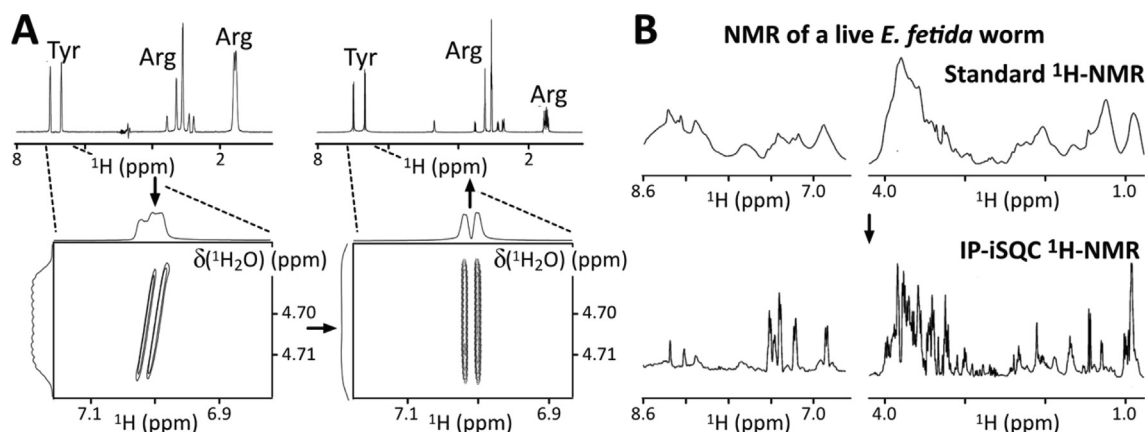
Fig. 33. A) Operating principle of intermolecular single-quantum correlation spectroscopy (iSQC), which correlates solute and water local resonance frequencies resonances and therefore allows a post-acquisition correction yielding an “inhomogeneity-free” final spectrum; ^1\text{H} -NMR spectra were recorded with a de-shimmed sample containing Tyrosine and Arginine; B) ^1\text{H} -NMR spectra of a live earthworm E. fetida recorded with a standard presaturation W5-WATERGATE pulse sequence (upper panel), and the IP-iSQC pulse sequence (lower panel) [1686]. Adapted from [1686].
