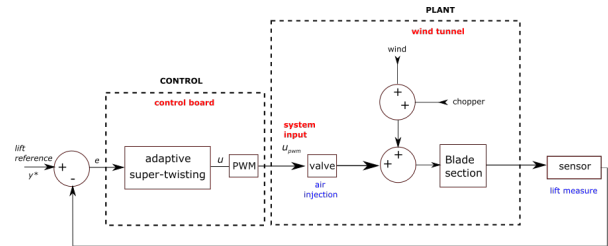
Fig. 6: Closed-loop scheme.
