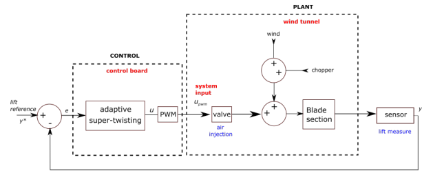
Fig. 6: Closed-loop scheme.
