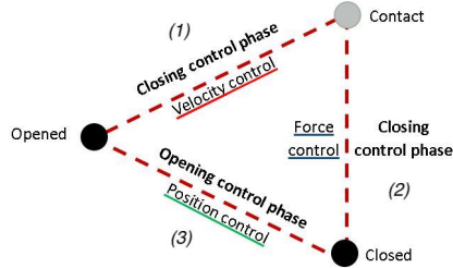
Fig. 1. Control phases between the open and closed positions.
