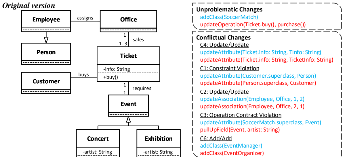
Figure 9: Experiment 1: original version of event management system and changes applied by two modelers (adapted from [31])
