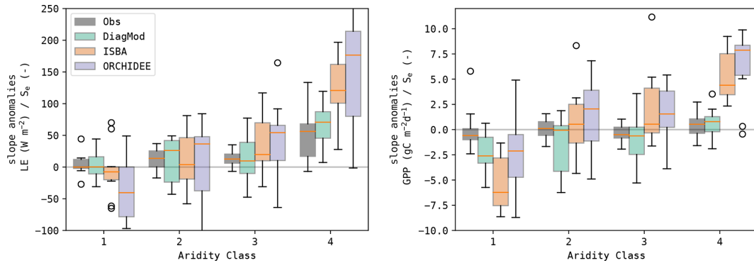
Figure 12. Boxplots of the slope of the linear regression between the anomalies in the state variables ( S_e and LAI) and the fluxes ( LE and GPP ) at the test sites, grouped per aridity class (1: least frequent drought stress; 4: most frequent drought stress).
