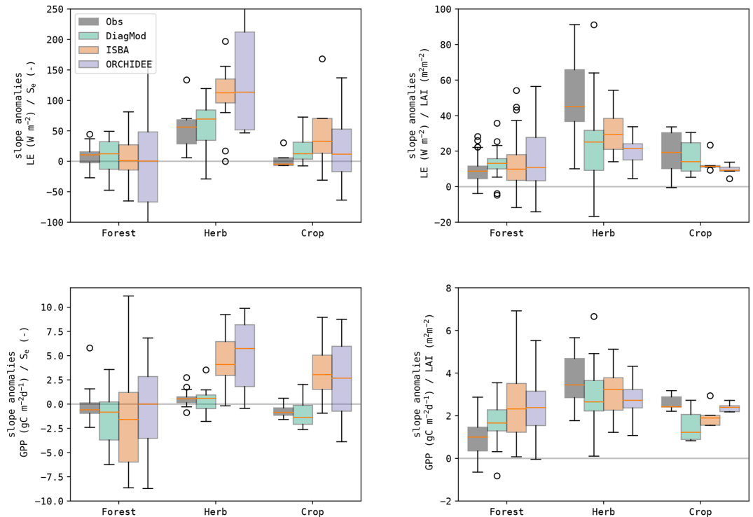
Figure 11. Boxplots of the slope of the linear regression between the anomalies in the state variables ( S_e and LAI) and the fluxes ( LE and GPP) at the test sites, grouped per dominant land cover.
