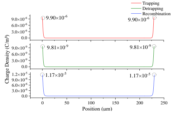
FIG. 3. Space charge densities involved in trapping, detrapping, and recombination in a voltage cycle (0.02 s) within 60 min with symmetrical parameters.
