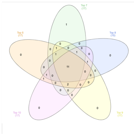
FIGURE S6. VENN DIAGRAMS OF THE OVERLAP OF INDIVIDUALS OF DIFFERENT MULTI-DIMENSIONAL PATTERNS FOR A SAME CATEGORY
