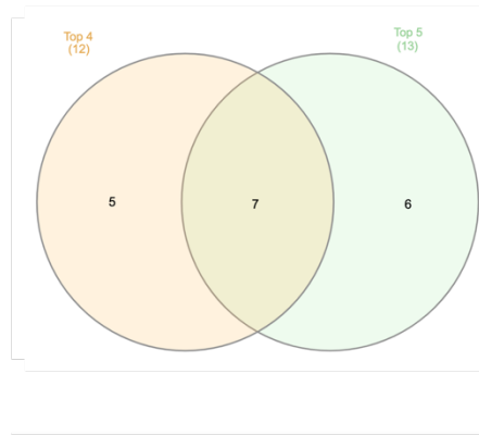
FIGURE S6. VENN DIAGRAMS OF THE OVERLAP OF INDIVIDUALS OF DIFFERENT MULTI-DIMENSIONAL PATTERNS FOR A SAME CATEGORY
