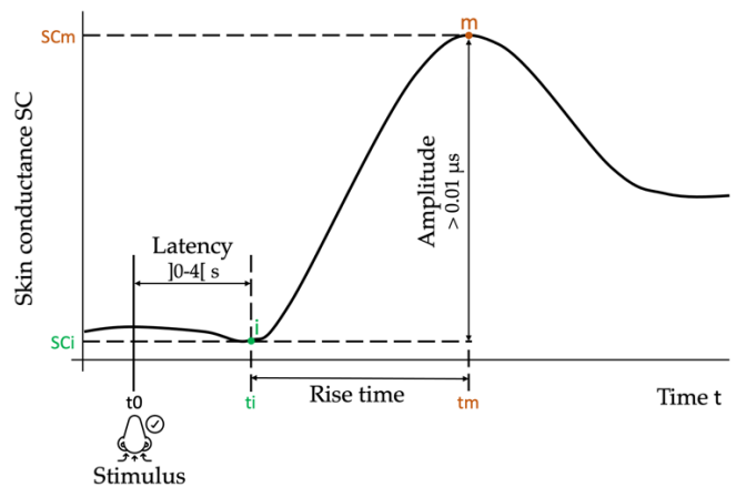
Fig. 2. Physiological attributes of the electrodermal response following stimulus presentation: latency (ms), rise time (ms), amplitude ( \mu S). t_0 corresponds to the time-point of odor presentation, i is the initiation point of the SC response and m is the maximum point of the SC response. The amplitude minimum is 0.01 \mu S and the initiation point is sought within the first 4 seconds. The calculation of the 3 variables is as follows: Latency = t_0 - t_i , Rise Time = t_m - t_i , Amplitude = SC_m - SC_i .
