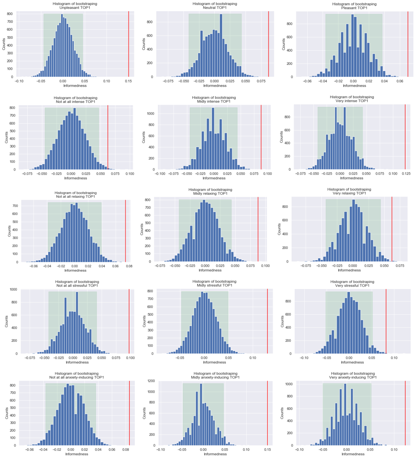
FIGURE S2. BOOSTRAPPING DISTRIBUTIONS FOR THE TOP1 PATTERN OF EACH DIMENSION AND EACH CLASS
