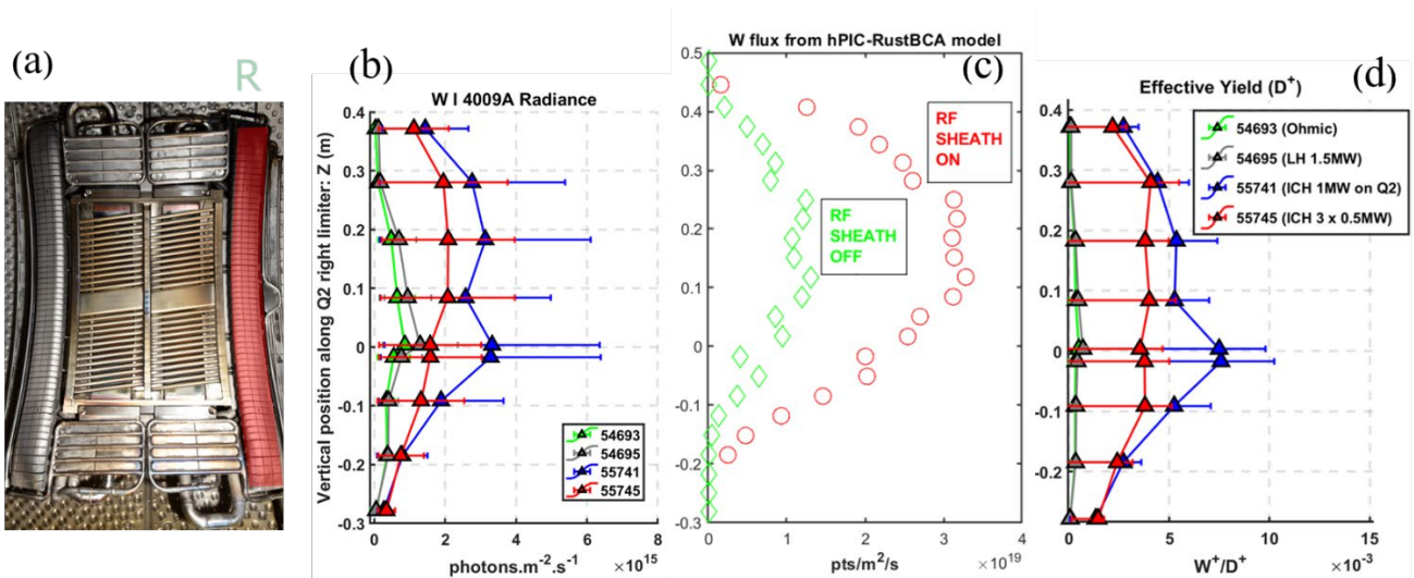
Figure 12. (a) Image of ICRH Antenna 2 with IC2R limiter highlighted; (b) measurements for ICRH-only shots, on similar target plasmas as the LH-only shots of Fig. 3, super-imposed with the latter; (c) a first simulation using hPIC-RustBCA with added RF sheath effect, specifically for the case of WEST Shot 55741, and assuming 100V peak-to-peak near-field at the observed limiter; (d) a D^+ effective yield particularly emphasizing the impact of the RF sheath on erosion for this shot with all the ICRH power applied to the observed antenna (Shot 55741).
