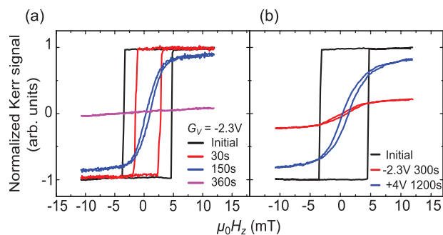
Figure 4. pMOKE hysteresis loops measured in sample S3 ( 350\text{ }^\circ\text{C} , zero dwell time) showing an SRT induced by the exposure to a gate voltage of -2.3\text{ V} for a) 360 s, and b) partial reversibility of the IP magnetized state after exposure to +4\text{ V} for 1200 s.
