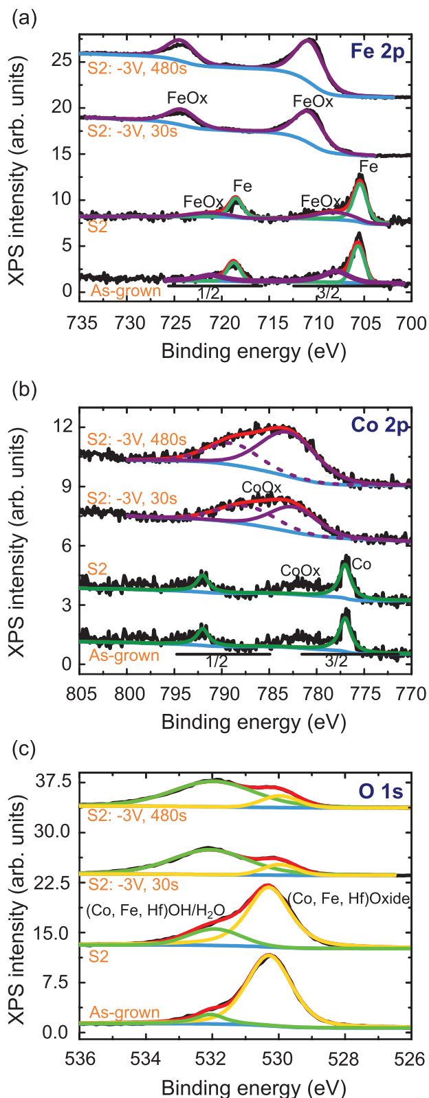
Figure 3. XPS spectra of a) Fe 2p 3/2 and 2p 1/2 , b) Co 2p 3/2 and 2p 1/2 , and c) O 1s for as-grown samples, S2, and S2 exposed to -3\text{ V} for 30 and 480 s. Raw data (black), total fitting (red), background (blue), and fitting of each peak: light green and yellow for O 1s peaks; dark green for Co and Fe 2p, and purple (dashed and solid) for oxides of Fe and Co 2p.
