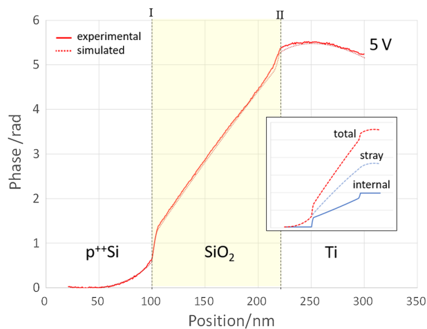
FIG. 3. Finite element method modeling of electric potential in sample device. Experimental phase profile for 5 V bias (red line), best fitting simulation (red dotted line). Inset: simulated phase contributions from internal potential (blue line), stray field (blue dotted line), and total (red dotted line). Potential steps at interfaces caused by dielectric charge layers.
