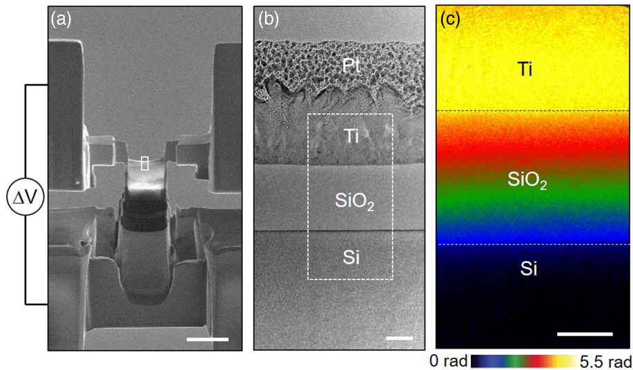
FIG. 1. Operando electron holography of nanocapacitor. (a) Scanning electron microscopy (SEM) image of specimen device within the FIB showing Pt deposited contacts to chip gold electrodes. (b) TEM image of active region showing substrate highly doped silicon, dielectric layer of silicon-dioxide (120 nm), top electrode of Ti, and Pt contact layer. (c) Phase map of projected electric potential obtained by electron holography [dotted region in (b)]. Scale bars are 5 \mu\text{m} for (a) and 50 nm for (b) and (c).
