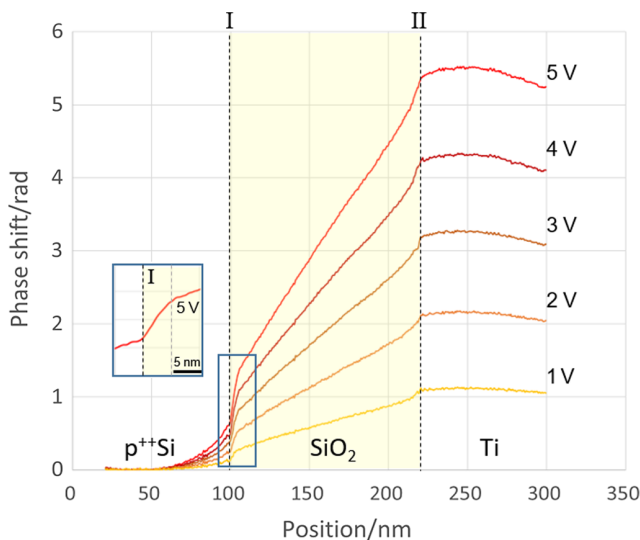
FIG. 2. Phase profiles as function of applied bias (1–5 V). Note the curvature of the phase within the electrodes (highly doped Si and Ti) and the phase jumps at the electrode-dielectric interfaces extending more than 5 nm inside the SiO _2 layer (see enlargement for 5 V bias).
