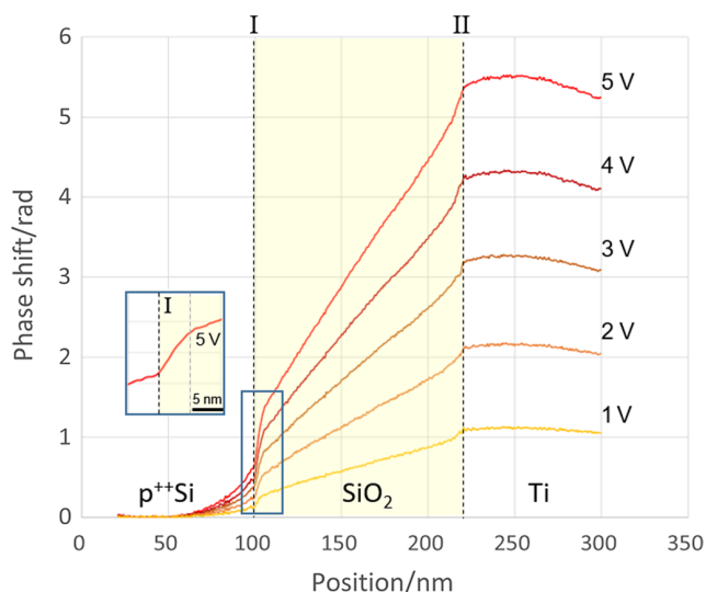
FIG. 2. Phase profiles as function of applied bias (1–5 V). Note the curvature of the phase within the electrodes (highly doped Si and Ti) and the phase jumps at the electrode-dielectric interfaces extending more than 5 nm inside the SiO 2 layer (see enlargement for 5 V bias).
