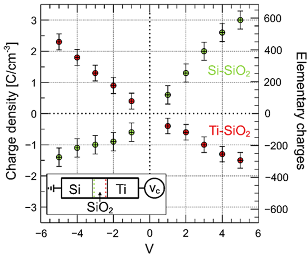
FIG. 4. Dielectric charge as a function of applied bias at Si-SiO 2 and SiO 2 -Ti interfaces. Left-hand axis in charges per unit volume. Right-hand axis in number of elementary charges contained in the analyzed region in the experimental specimen device.
