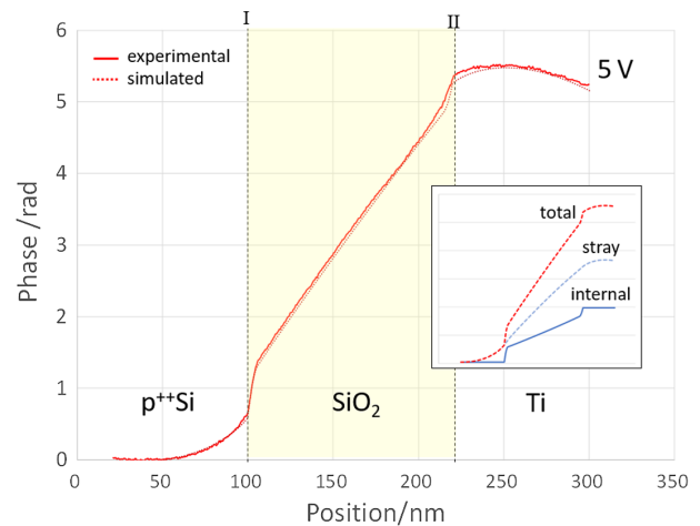
FIG. 3. Finite element method modeling of electric potential in sample device. Experimental phase profile for 5 V bias (red line), best fitting simulation (red dotted line). Inset: simulated phase contributions from internal potential (blue line), stray field (blue dotted line), and total (red dotted line). Potential steps at interfaces caused by dielectric charge layers.
