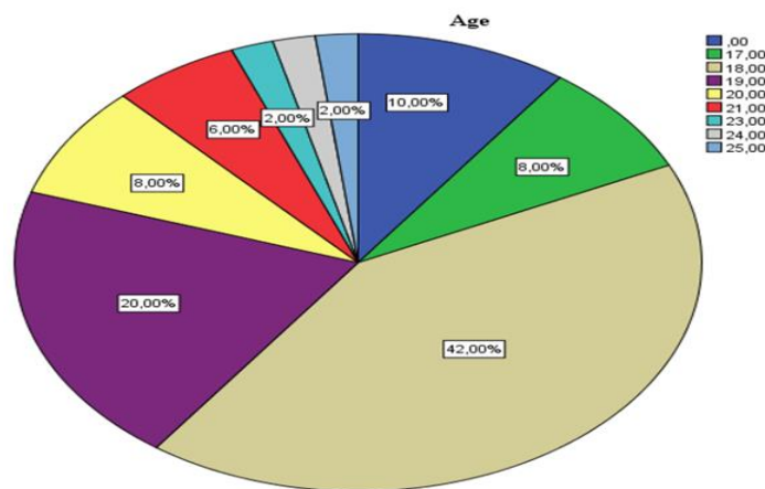
Figure 2 Participants' Age
