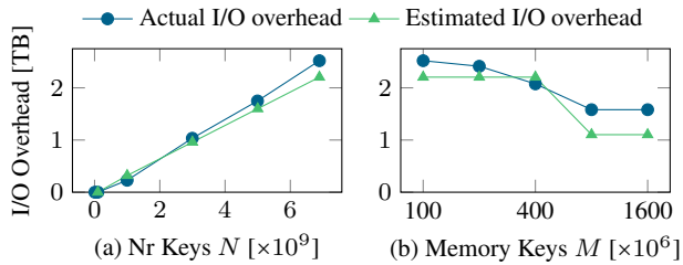
Fig. 17: Bulk-Loading cost model
