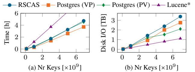
Fig. 15: Bulk-Loading performance
