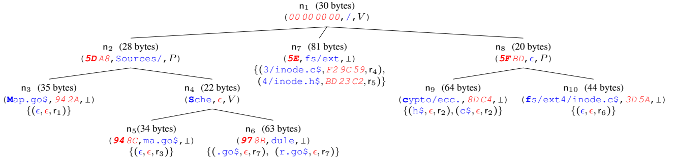
Fig. 4: The RSCAS trie for the composite keys K^{1..9} .
