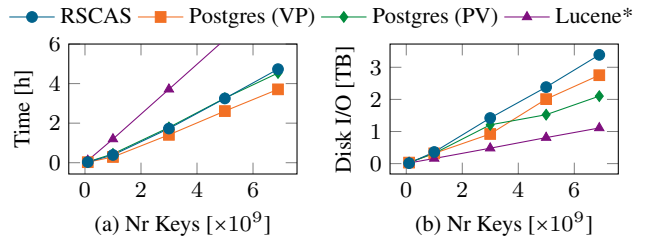
Fig. 15: Bulk-Loading performance
