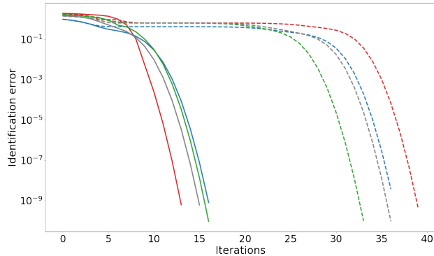
Fig. 1: Identification error on identifying the matrices A and B with Q = 10^{-4}I_n . Pairs of curves with the same colors are identification experiments on the same problem parameters solved using different solvers: diff-mpc in dashed lines and ours in solid lines. The same convention is used in all figures.
