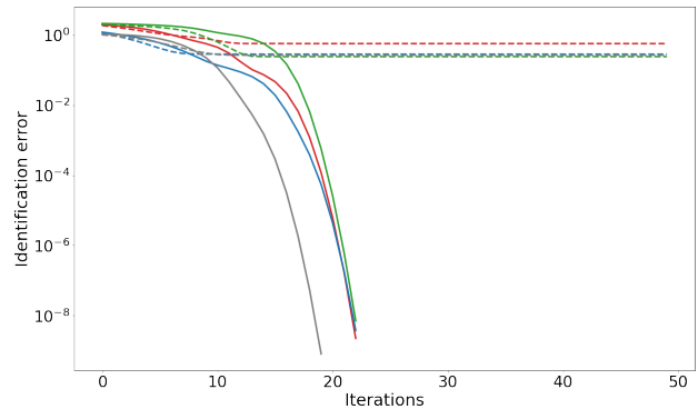
Fig. 3: Identification error . Identification of Q .
