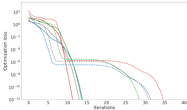
Fig. 2: Optimization loss on identifying the matrices A and B with Q = 10^{-4}I_n .
