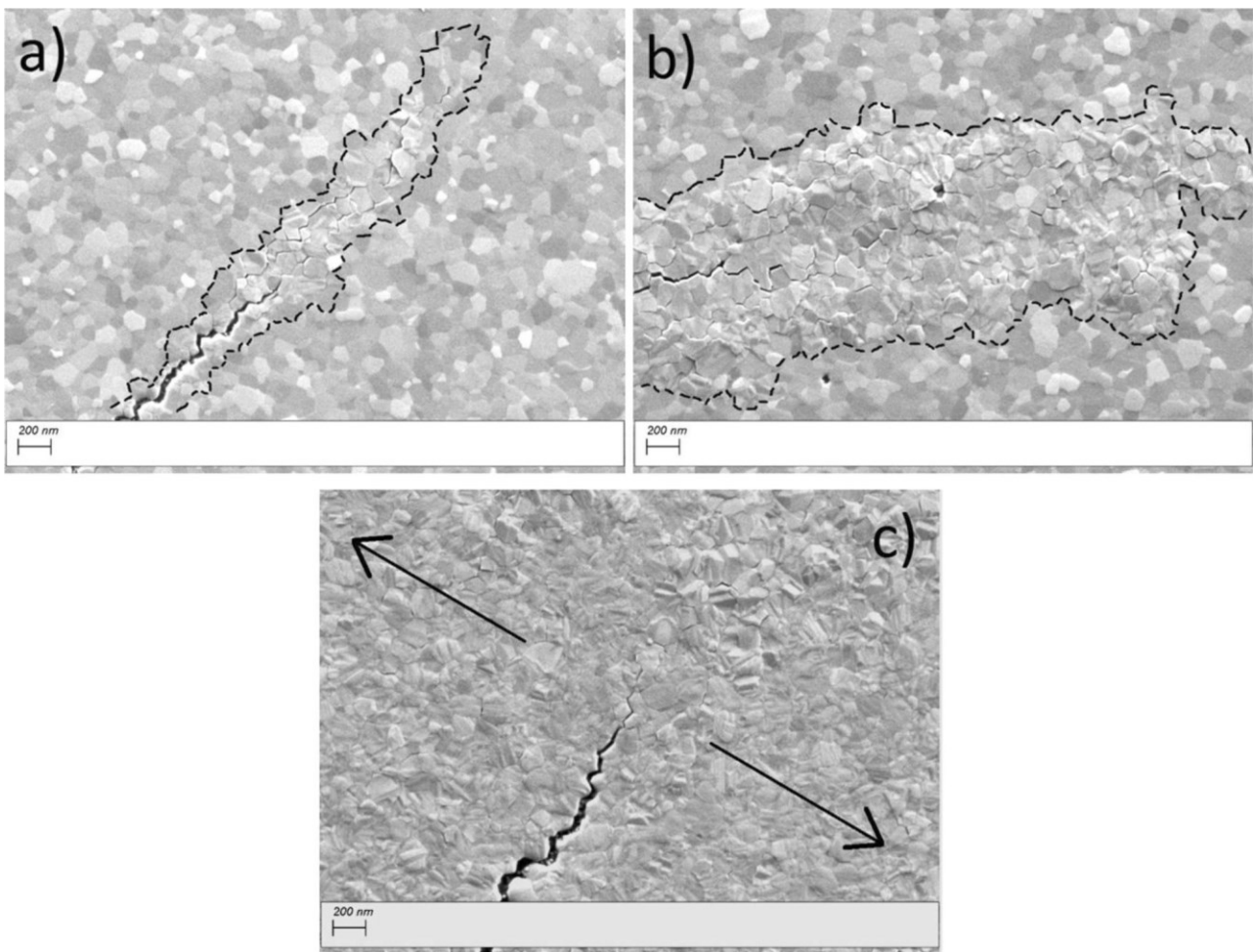
Figure 7: Vicinity of indentation cracks in tetragonal YSZ with grain size of 75 \pm 5 nm; a) 3YSZ, b) 2YSZ, and c) 1.5YSZ. Dash-lines in (a) and (b) highlight the boundary of transformed zone around the crack. Arrows in (c) shows the width of transformed zone around the crack.
