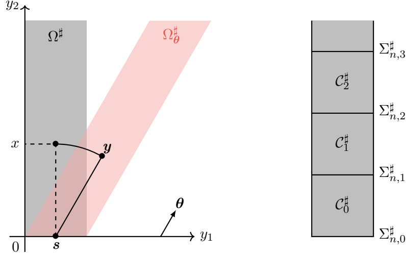
Figure 5: The half-cylinders \Omega^\sharp and \Omega_\theta^\sharp (left), and the domains C_\ell^\sharp and \Sigma_{n,k}^\sharp (right) for n = 2 as well as the one-dimensional problems
