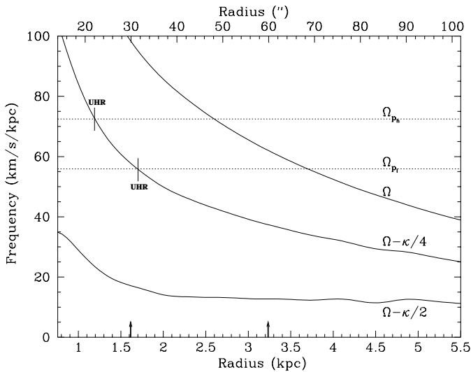
Fig. 6. Angular velocities in NGC 3627 as function of radius. The dotted horizontal lines indicate a bar pattern speed of, respectively, 56 \text{ km s}^{-1} \text{ kpc}^{-1} ( \Omega_{\text{pl}} ) and 72 \text{ km s}^{-1} \text{ kpc}^{-1} ( \Omega_{\text{pb}} ), giving an ultraharmonic resonance between 1.2 and 1.7 kpc radius, with the \Omega - \kappa/4 curve. The arrows indicate the extension of the annular structure in the galaxy, between 30'' and 60'' .
