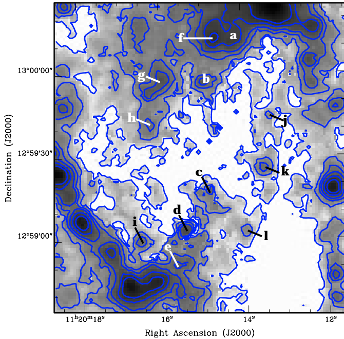
Fig. 2. Enlarged H\alpha image of the inner regions of NGC 3627 from Fig. 1d. Contours of the smoothed H\alpha map are at confidence levels of (3, 10.5, 22, 37, 57, 76) \times \sigma_{\text{mono}} above the mean monochromatic background level ( \sigma_{\text{mono}} represents the dispersion around this mean level in arbitrary units) and superimposed on a grey-scale representation of the same H\alpha image. The letters indicate the positions of some HII regions along the leading sides of the bar and in the H\alpha arclets (see text for details).
