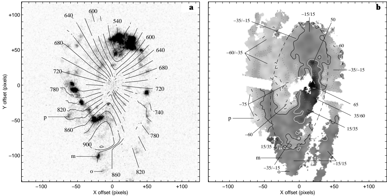
Fig. 5. a) Model velocity field superimposed on our high-resolution H \alpha image. Velocity contours are separated by 20 km s ^{-1} . b) Grey-scale representation of the residual velocity field (observation minus model). The dashed ellipse represents the R = 88'' limit between the axisymmetric model and the tilted-ring outer disc models. In each image, the [0,0] point refers to the kinematical centre and the letters “m”, “o” and “p” to HII regions discussed in the text.
