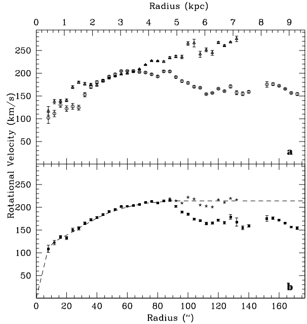
Fig. 3. H\alpha rotation curve of NGC 3627. a) The rotation curves of the approaching and the receding sides fitted separately: open circles and triangles are for the receding and approaching sides respectively. b) The global rotation curve, fitted to both sides of the disc (squares). Stars indicate the average of the receding and the approaching sides curves at radii above 88'' . The dashed line shows the adopted best model for the global rotation curve.
