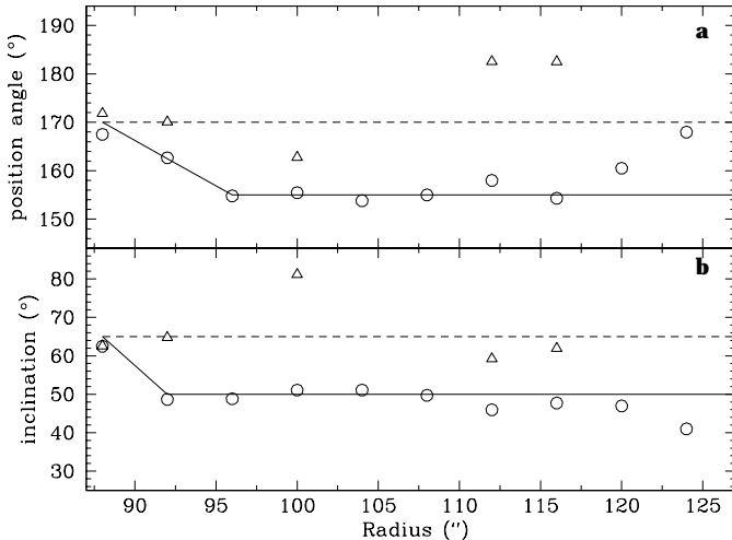
Fig. 4. Position angle a ) and inclination b ) as function of deprojected galactocentric radius, starting from R = 88'' . Open circles and the solid line represent the fitted points and the adopted model parameters for the receding side, while open triangles and the dotted line show the same quantities for the approaching side.
