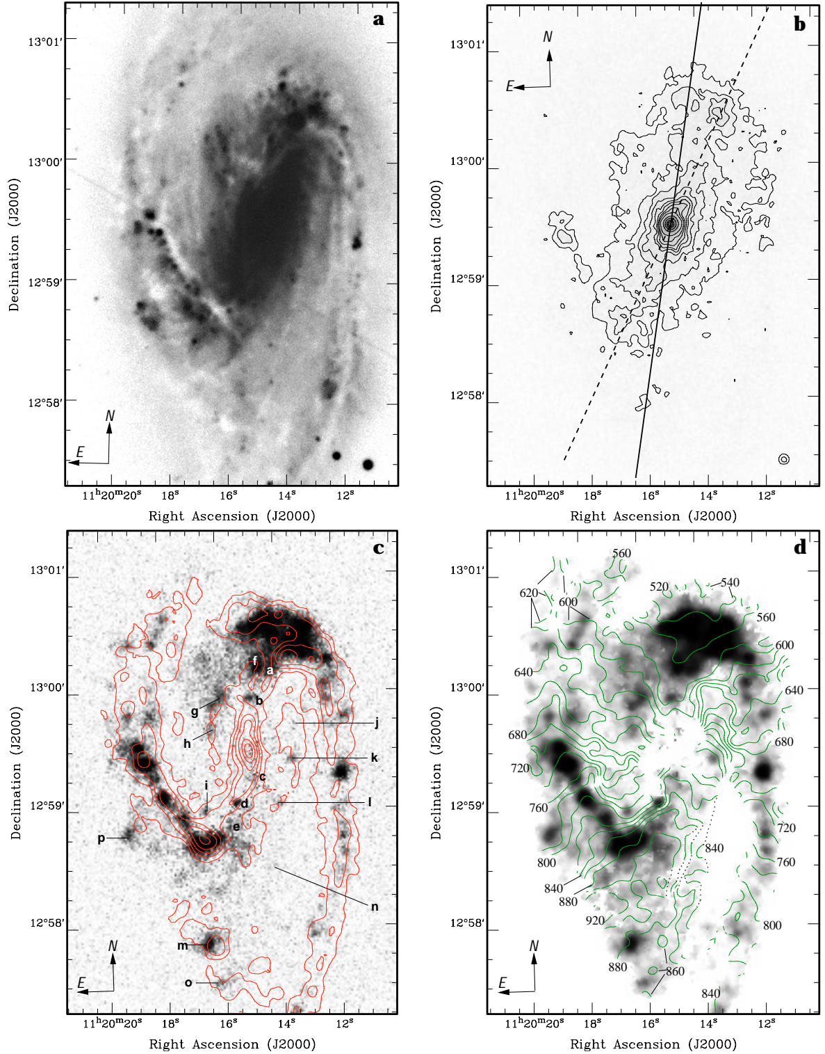
Fig. 1. a) Optical broad-band image of NGC 3627, taken from the Anglo Australian Observatory’s website. b) Continuum map of NGC 3627 from our observations. The contour levels are at (3, 5, 7, 9, 11, 13, 15, 17, 21, 31, 42, 52, 57) \times \sigma_{\text{cont}} above the mean continuum background level ( \sigma_{\text{cont}} represents the dispersion around this mean level in arbitrary units). The solid line indicates the direction of the kinematical major axis of the galaxy and the dashed line indicates the direction of the major axis of the optical bar. c) Grey scale image (full resolution) of the H\alpha integrated emission line of NGC 3627 with superimposed CO(1–0) intensity contours (Regan et al. 1999) with levels of (4, 12, 26, 50, 90, 130, 170) \text{Jy/beam} \times \text{km s}^{-1} . The letters indicate the positions of HII regions along the leading sides of the bar, in the H\alpha arcs and in the interstellar medium (see text for details). d) Isovelocity contours of our H\alpha velocity field superimposed on a smoothed (by 3 \times 3 pixels FWHM ) greyscale of our H\alpha integrated brightness. The contour levels are separated by 20 \text{ km s}^{-1} .
