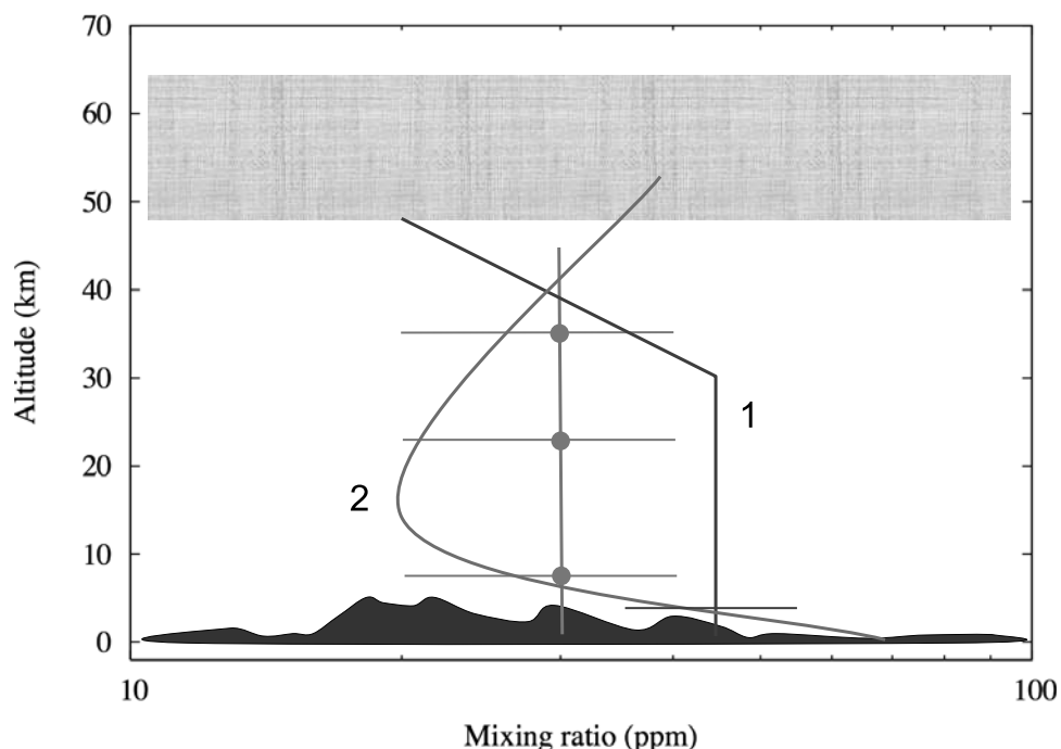
Figure 9. Determination of the H 2 O mixing ratio profile from various investigations. Dots with error bars: night-side observations as compiled by Taylor et al. [1997]. 1, Meadows and Crisp's [1996] AAT night-side observations; 2, Ignatiev et al.'s [1997] reanalysis of the Venera optical spectra.
