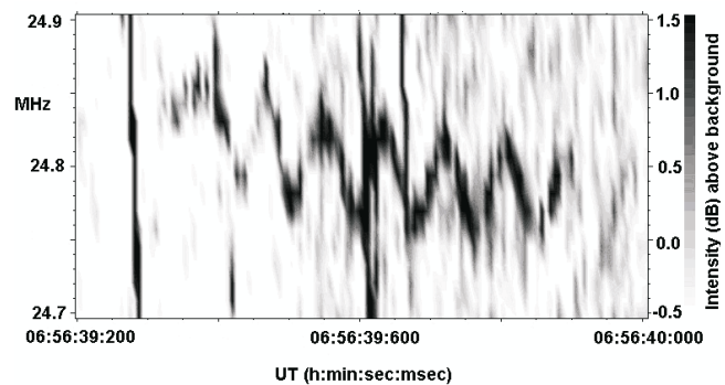
Fig. 10. Specific spectrum (Io-A source) which consists of frequency drifting consecutive quasi-harmonic structures against a background of classical S-burst emission (top), zoom-in fragment (bottom).
