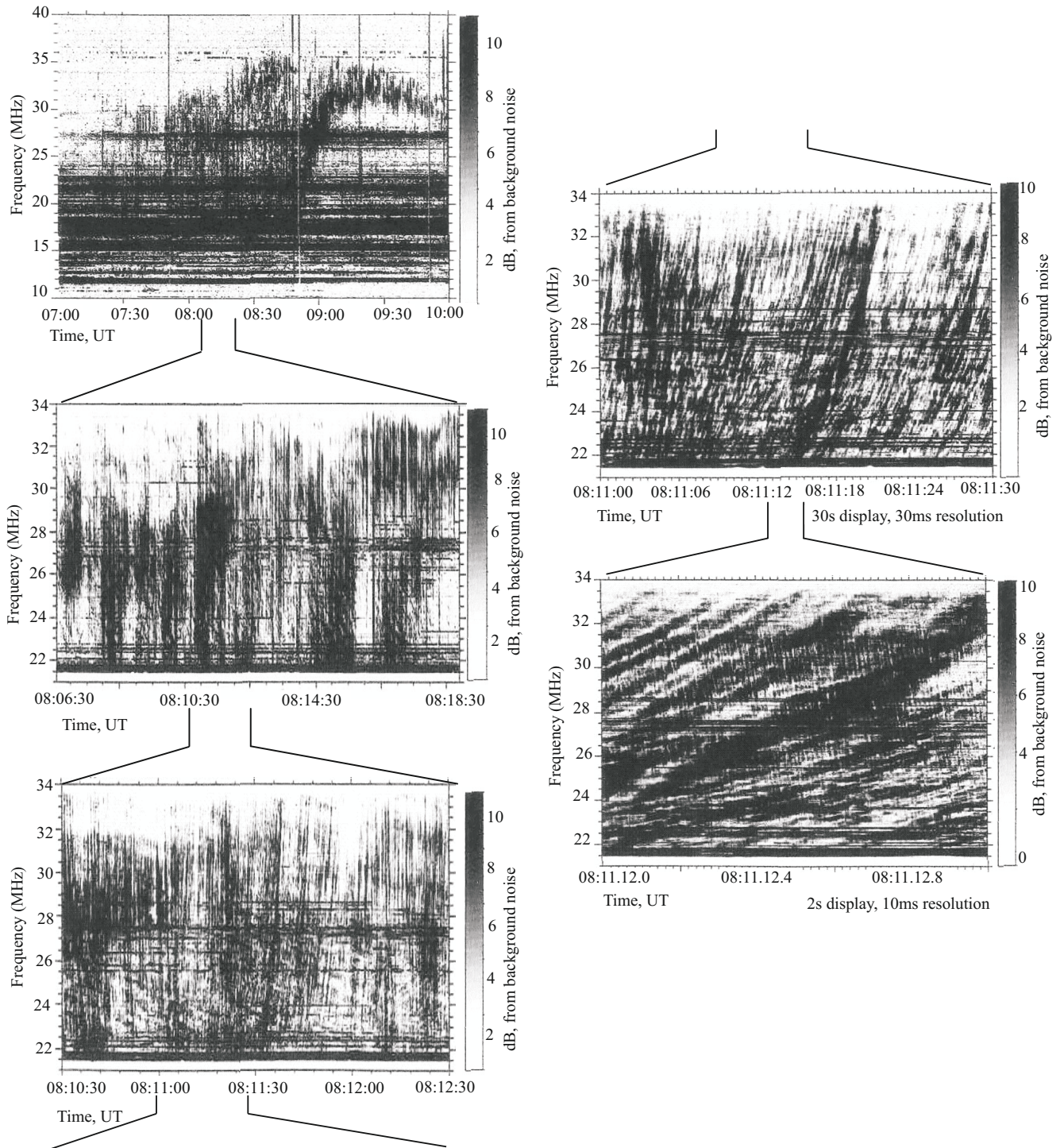
Fig. 1. Images of the Jovian DAM emission spectra on different time scales (NDA + DSP, Io-B source).
