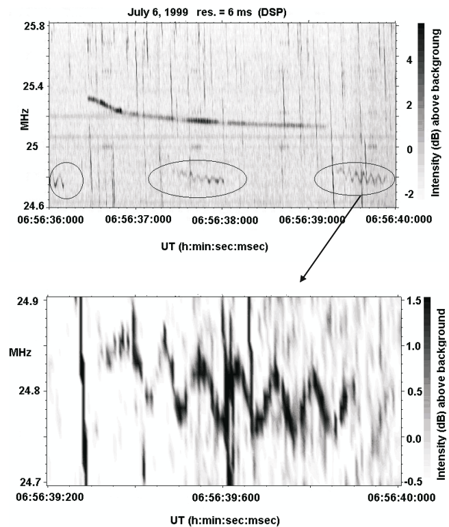
Fig. 10. Specific spectrum (Io-A source) which consists of frequency drifting consecutive quasi-harmonic structures against a background of classical S-burst emission (top), zoom-in fragment (bottom).
