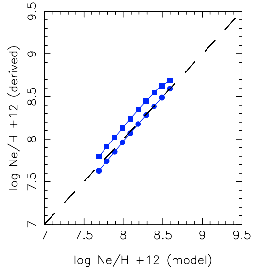
Fig. 11. The \text{Ne}/\text{H} ratio derived by T_e -based methods for our model planetary nebulae as a function of input \text{Ne}/\text{H} values in our models.
