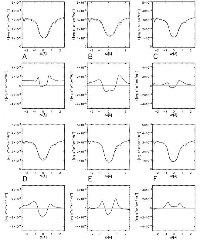
Fig. 10. THEMIS/MTR H\alpha profiles of the 6 EBs identified in Fig. 9. For each EB – Upper panels: bold line: EB profile; dashed line: nearby reference H\alpha profile. Bottom panels: EB profiles in the H\alpha line, with the nearby profile subtracted.
