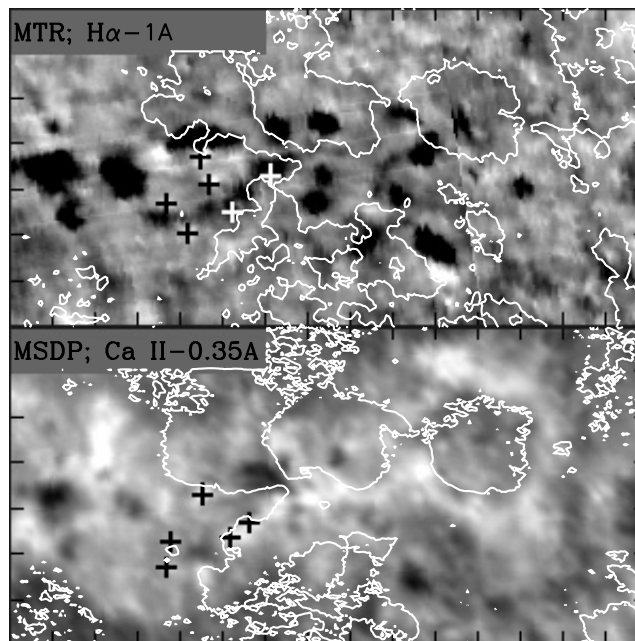
Fig. 11. Top panel: THEMIS/MTR H\alpha observations at -1 \text{ \AA} from the first scan (10:33–11:30 UT). The isocontours correspond to the null value of the Stokes V parameter (from Fe I 6302 \text{\AA} line) and thus to the neutral line of the longitudinal magnetic field. The 6 crosses locate the position of some EBs presented in Fig. 9. Bottom panel: THEMIS/MSDP Ca II -0.35 \text{ \AA} observation at 8:27 UT. The isocontours correspond to the inversion lines of the longitudinal field derived from Na D1. The 5 crosses correspond to the position of the 5 EBs that can be related to those observed in H\alpha with MTR mode, about 2 h later.
