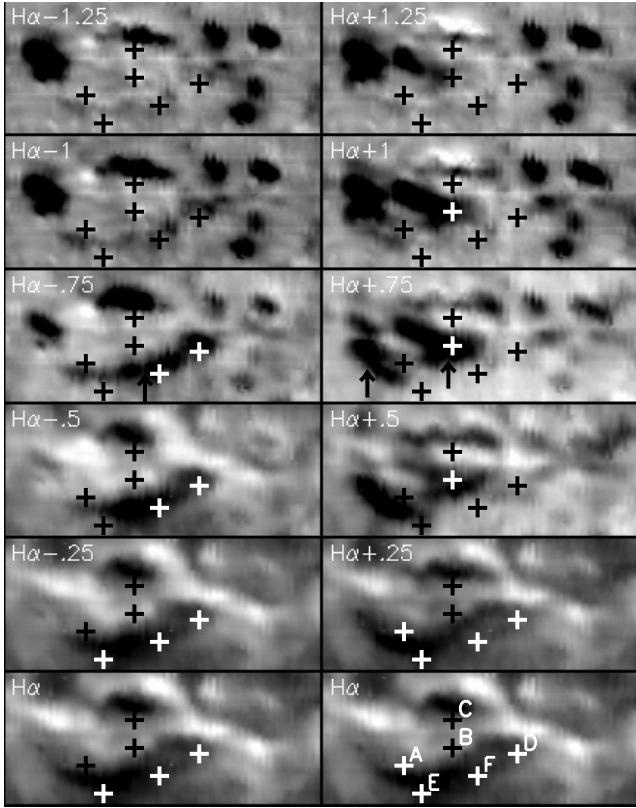
Fig. 9. THEMIS/MTR observations of the NOAA 10655 on August 3, 2004 between 10:33 UT and 11:30 UT (first scan) on the H\alpha line. Several EBs have been located by a plus sign and labeled from “A” to “F”. The field-of-view of these images is 72'' \times 31'' and corresponds to the area enclosed in the black rectangle of Fig. 5. Left panels: blue wing of H\alpha . The dark structures (like the one indicated with an arrow in the H\alpha -0.75 \text{ \AA} image) correspond to the top of rising arch filaments. Right panels: red wing of H\alpha . We note downflows within the arch filaments legs (for example those indicated by arrows in the H\alpha +0.75 \text{ \AA} image).
