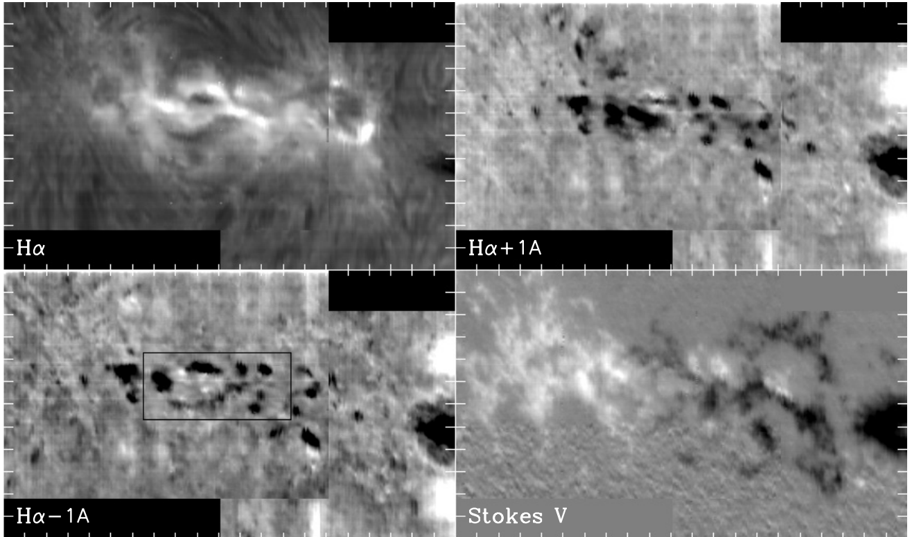
Fig. 5. THEMIS/MTR observations of the NOAA 10655 on August 3, 2004 between 10:33 UT and 12:22 UT. The field-of-view of these images is 218'' \times 122'' : H\alpha center line (top left panel), at +1 \text{ \AA} (top right panel), and at -1 \text{ \AA} (bottom left panel). The field-of-view of all the images is perfectly co-spatial due to the ability of MTR to observe several lines simultaneously. Stokes V map determined from Fe I line (bottom right panel). The black rectangle in the bottom left panel indicates the emerging flux region where several AFs are visible (in the H\alpha line center image, top left panel) and where several EBs occur (see bright points at H\alpha -1\text{\AA} , bottom left panel).
