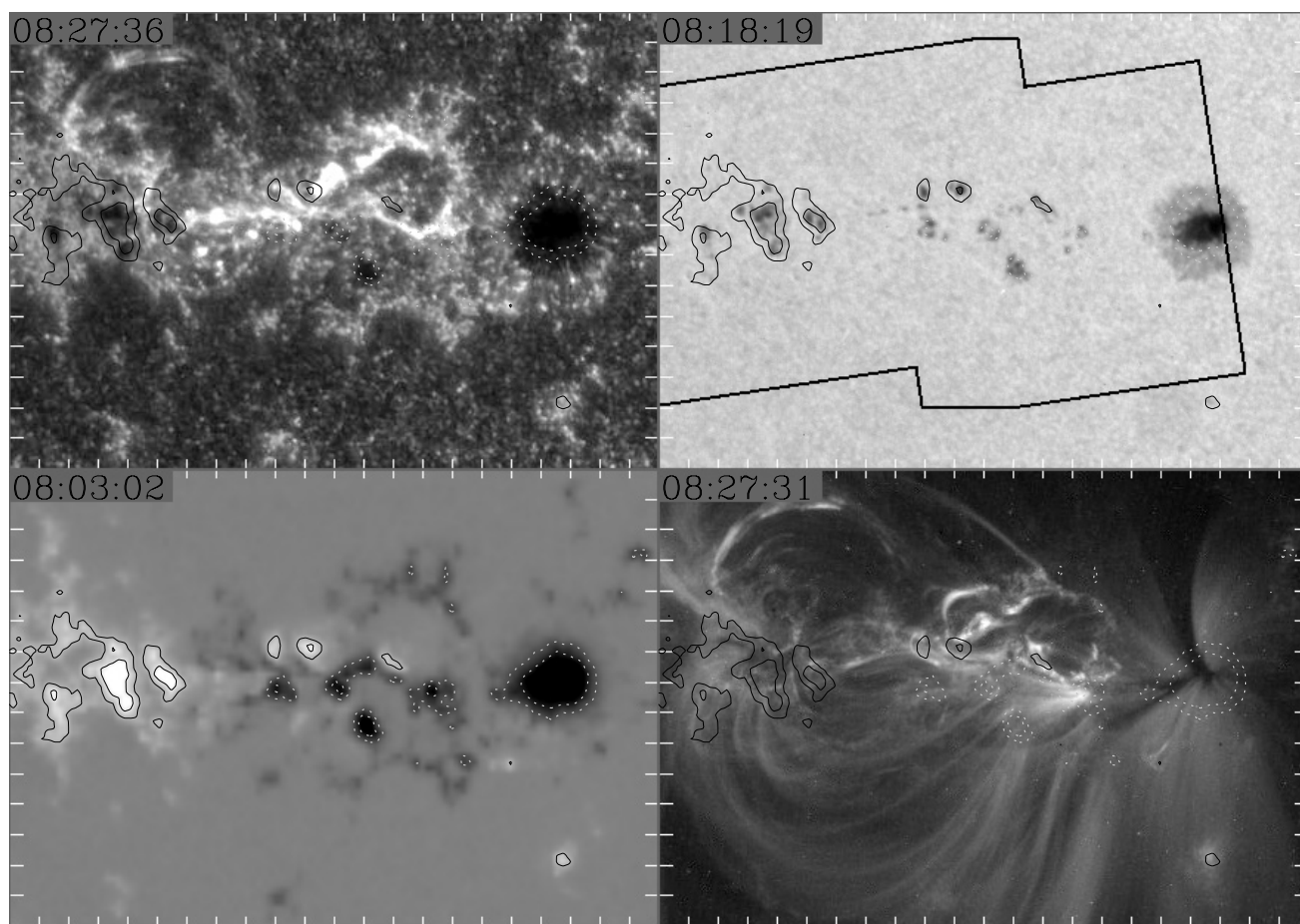
Fig. 1. Images of the active region NOAA 10655 obtained nearly simultaneously on August 3, 2004. TRACE 1600 Å ( top left ) and white-light ( top right ) images. The field of view of the THEMIS/MTR scans is represented in the white light image (thick solid line). SoHO/MDI map of the longitudinal magnetic field ( bottom left ) and TRACE 195 Å image ( bottom right ). The isocontours in each panel are those of the longitudinal magnetic field obtained with SoHO/MDI of \pm 300, 600 Gauss.
