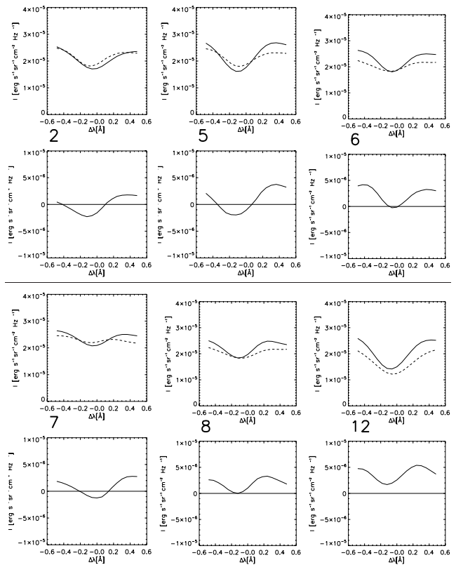
Fig. 8. Ca II 8542 Å profiles of EBs in areas “2”, “5”, “6”, “7”, “8”, and “12” observed at 08:36–08:43 UT. For each EB – Upper panels: bold line: EB profile; dashed line: reference nearby Ca II line profile. Bottom panels: EB profiles in the Ca II line, with the nearby profile subtracted.
