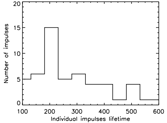
Fig. 7. Histogram of the lifetime of the individual impulses in the EB time profiles observed by TRACE at 1600 Å for the active region NOAA 10655 between 08:11 UT and 08:51 UT. The axis of ordinates corresponds to the number of impulses which lifetime (in second) is given in the axis of abscissas, binned by a factor of 50 s.
