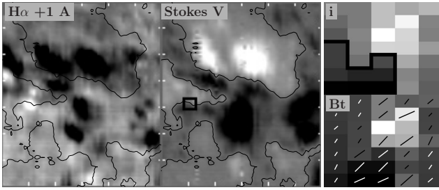
Fig. 12. Left: H\alpha image at \pm 1 \text{ \AA} from the second MTR scan (11:37–12:22 UT) of the emerging flux area. Middle: location (black box) of the EB “D” (see Fig. 9) on the Stokes V map. The field-of-view of these images is 40'' \times 47'' . The isocontours correspond to the null value of the Stokes V parameter. Note that around the EB, the inversion line presents some undulations, in the form of “~”, in the vicinity of the black box, respective to the horizontal (left-right) direction. Right down: longitudinal magnetogram around the EB. The field-of-view of this image is 4'' \times 3.15'' and corresponds to the area within the black box in the middle panel. The segment gives the direction of the transverse field. The ambiguity has not been resolved. The length is proportional to the transverse field intensity. Right up: elevation angle i of the magnetic field (angle of the field relatively to the plane perpendicular to the line-of-sight), coded in levels of gray. White and light grays indicate positive values and thus the magnetic field pointing upward, and black and dark grays refer to negative values and correspond to the magnetic field pointing downward. The bold black line indicates the position of the inversion line. Note that its detailed shape strongly depends on the pixel size and resolution and cannot be directly interpreted.
