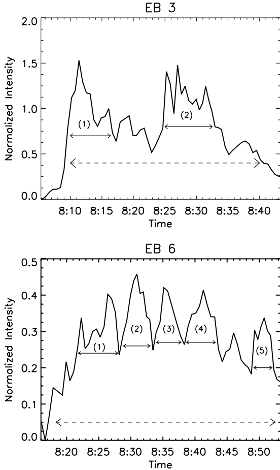
Fig. 6. Two examples of the time evolution of the brightness of EBs observed at 1600 Å (TRACE). These plots are for EB “3” (upper panel) and “6” (lower panel) (see Fig. 4). The axis of ordinates shows the normalized intensity: the absolute intensity divided by the minimum value minus one. The duration of the EB is indicated by dashed arrows. The EB time profiles present individual impulses (2 for EB “3” and 5 for EB “6”), whose lifetimes are indicated by continuous arrows.
