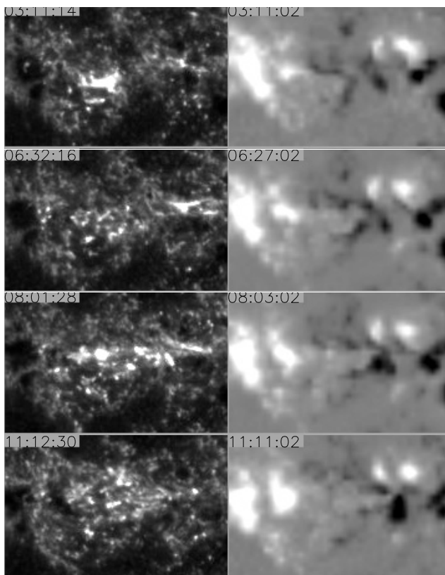
Fig. 3. Evolution of the eastern part of the active region NOAA 10655 observed on August 3, 2004 by TRACE at 1600 Å ( left column ) and the SoHO/MDI magnetograph ( right column ).
