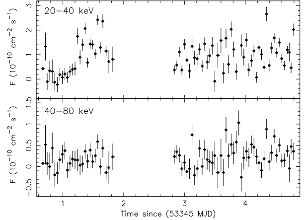
Fig. 2. INTEGRAL /ISGRI light curve of 2S 0114+65 in the 20–40 and 40–80 keV energy bands. The ISGRI data are taken from the whole observation and have been converted to flux assuming a power law with an exponential high-energy cut-off model (see Table 1). Each point corresponds to a \sim 2.2 ks interval.
