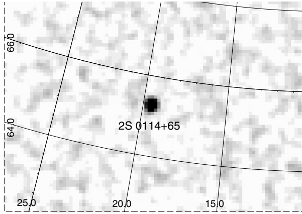
Fig. 1. The 20–40 keV IBIS/ISGRI mosaicked and deconvolved sky image of the \sim 182 ks observation. Image size is \sim 15^\circ \times 5^\circ , centered at 2S 0114+65 position. The pixel size is 5' . 2S 0114+65 was detected at a significance of \sim 37\sigma .
