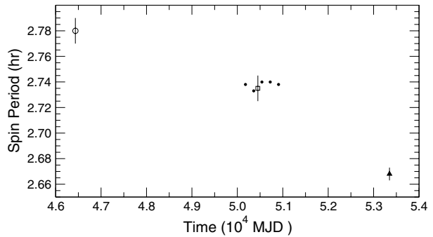
Fig. 4. Spin history of 2S 0114+65. The filled triangle is from this work. The open circle is from Finley et al. (1992), filled circles from Corbet et al. (1999), and open square from Hall et al. (2000).
