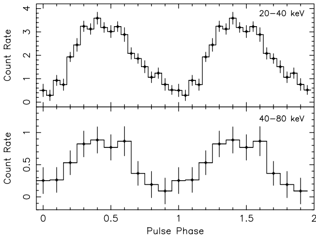
Fig. 3. IBIS/ISGRI background subtracted light curve of 2S 0114+65 folded at the best found NS spin period (2.668 h). The epoch T_0 is arbitrary. From top to bottom the energy ranges are 20–40 keV and 40–80 keV, respectively. The pulse profile is repeated once for clarity.
