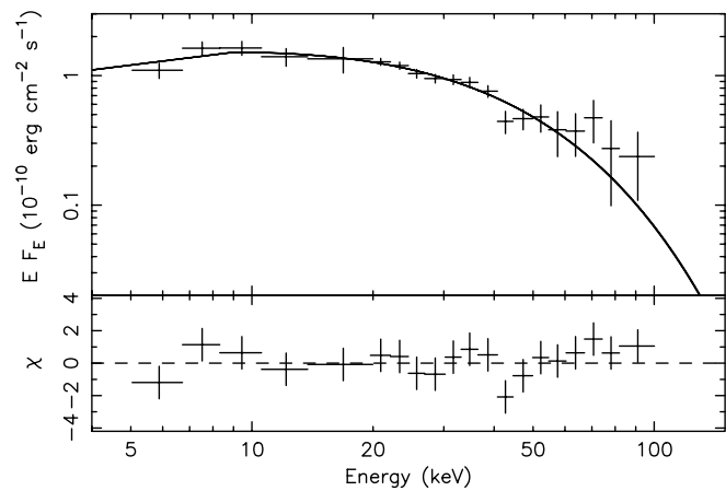
Fig. 5. INTEGRAL /JEM-X (5–20 keV) and ISGRI (20–100 keV) unfolded spectra of 2S 0114+65 with the best-fit power law and exponential high-energy cut-off model. Residuals between the data and model are shown in the bottom panel in units of sigma.
